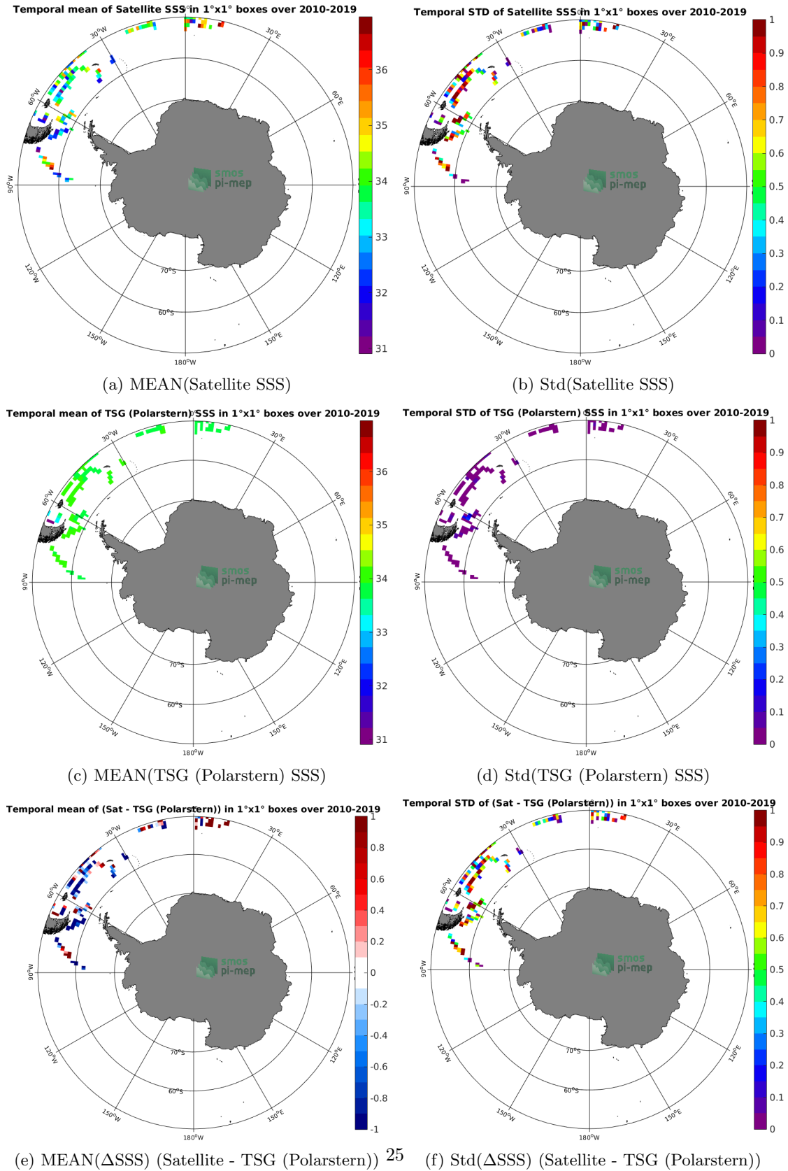
Figure 6: Temporal mean (left) and Std (right) of SSS from SMOS SSS L2 v662 (ESA) (top), TSG (Polarstern) (middle), and of \Delta SSS (Satellite - TSG (Polarstern)). Only match-up pairs are used to generate these maps.
