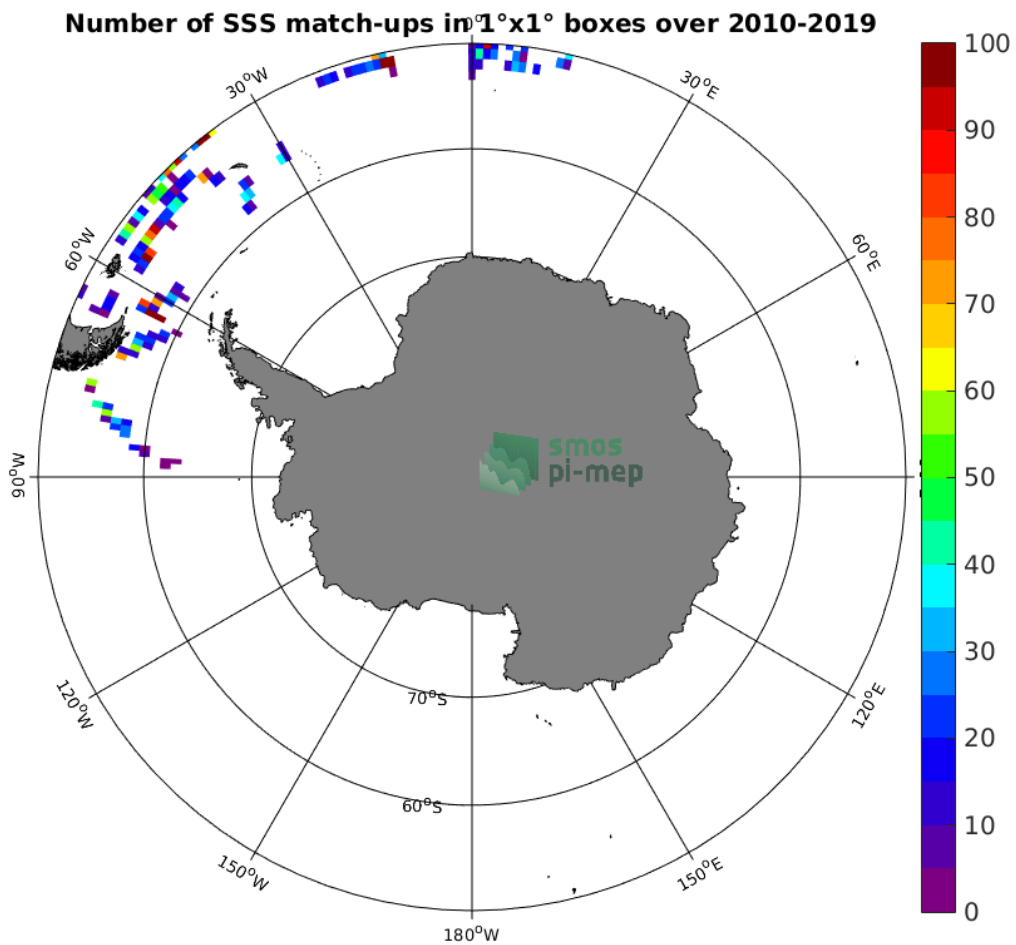
Figure 4: Number of SSS match-ups between TSG (Polarstern) SSS and the SMOS SSS L2 v662 (ESA) SSS product for the Southern Ocean Pi-MEP region over 1^\circ \times 1^\circ boxes and for the full satellite product period.
