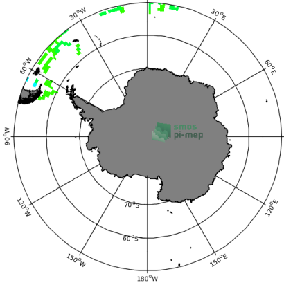
(c) MEAN(TSG-POLARSTERN SSS)
