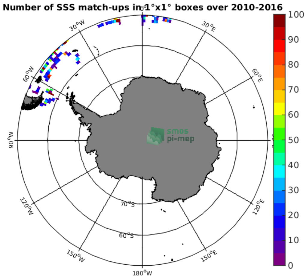
Figure 4: Number of SSS match-ups between TSG-POLARSTERN SSS and the SMOS-L2-DPGS-v662 SSS product for the Southern Ocean Pi-MEP region over 1°x1° boxes and for the full satellite product period.
