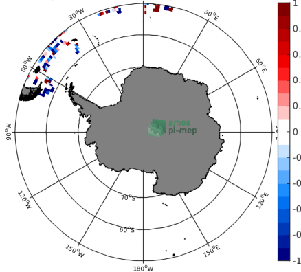
(e) MEAN( \Delta SSS) (Satellite - TSG-POLARSTERN)
