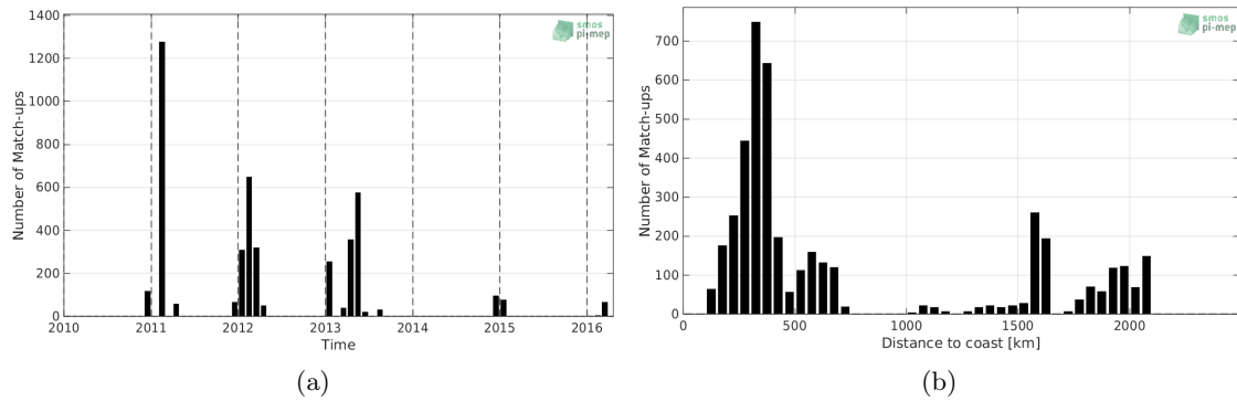
Figure 1: Number of match-ups between TSG-POLARSTERN and SMOS-L2-DPGS-v662 SSS as a function of time (a) and as function of the distance to coast (b) over the Southern Ocean Pi-MEP region and for the full satellite product period.
