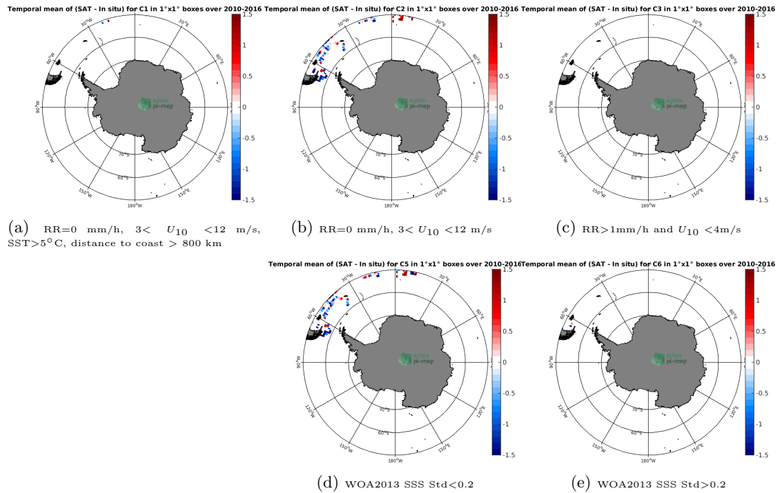
Figure 12: Temporal mean gridded over spatial boxes of size 1^\circ \times 1^\circ of \Delta SSS (SMOS-L2-DPGS-v662 - TSG-POLARSTERN) for 5 different subdatasets corresponding to: RR=0 mm/h, 3 < U_{10} < 12 m/s, SST > 5^\circ\text{C} , distance to coast > 800 km (a), RR=0 mm/h, 3 < U_{10} < 12 m/s (b), RR > 1 mm/h and U_{10} < 4 m/s (c), WOA2013 SSS Std < 0.2 (d), WOA2013 SSS Std > 0.2 (e).
