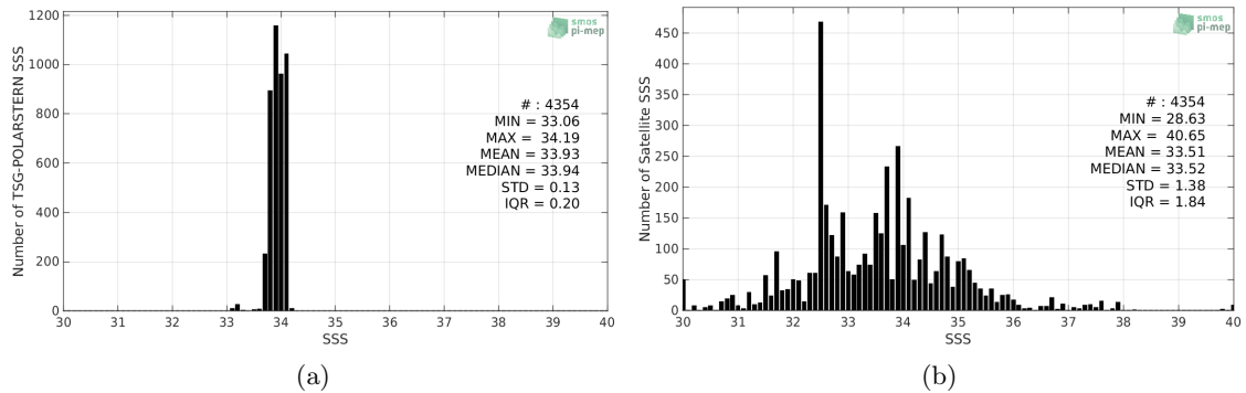
Figure 2: Histograms of SSS from TSG-POLARSTERN (a) and SMOS-L2-DPGS-v662 (b) considering all match-up pairs per bins of 0.1 over the Southern Ocean Pi-MEP region and for the full satellite product period.
