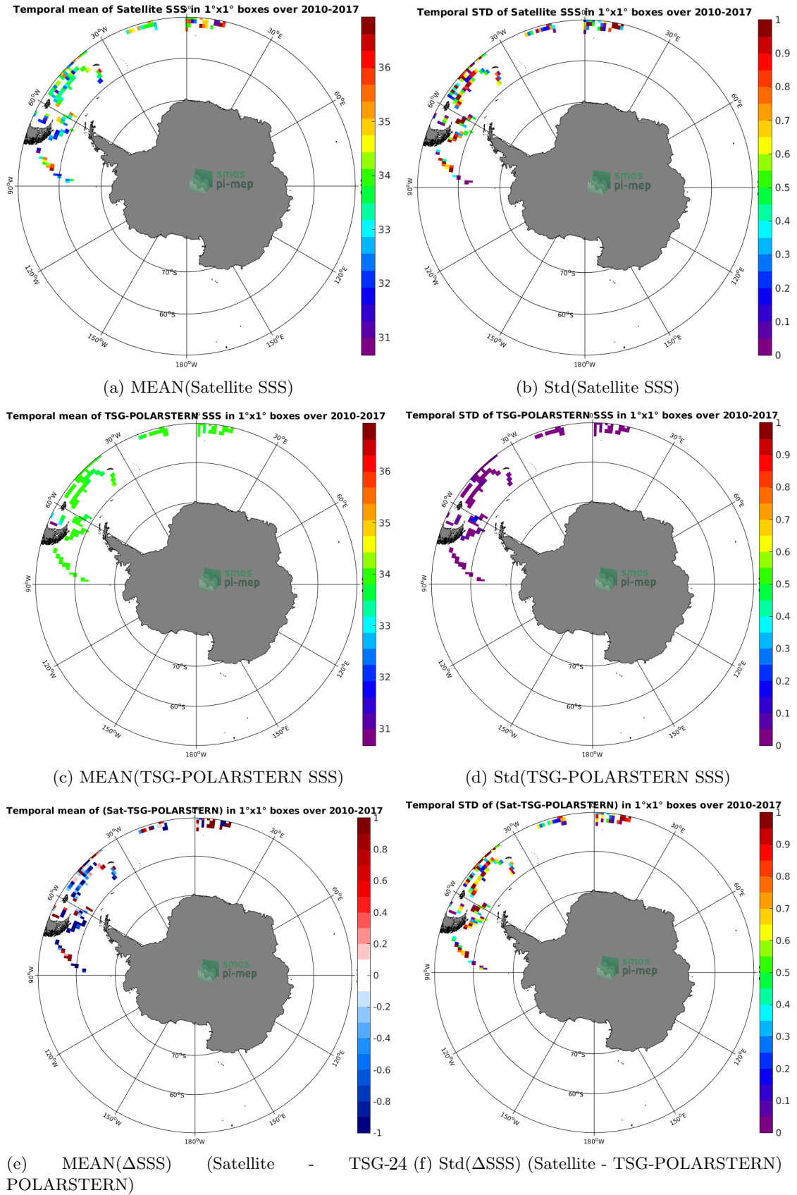
Figure 6: Temporal mean (left) and Std (right) of SSS from SMOS-L2-DPGS-v662 (top), TSG-POLARSTERN (middle), and of \Delta SSS (Satellite - TSG-POLARSTERN). Only match-up pairs are used to generate these maps.
