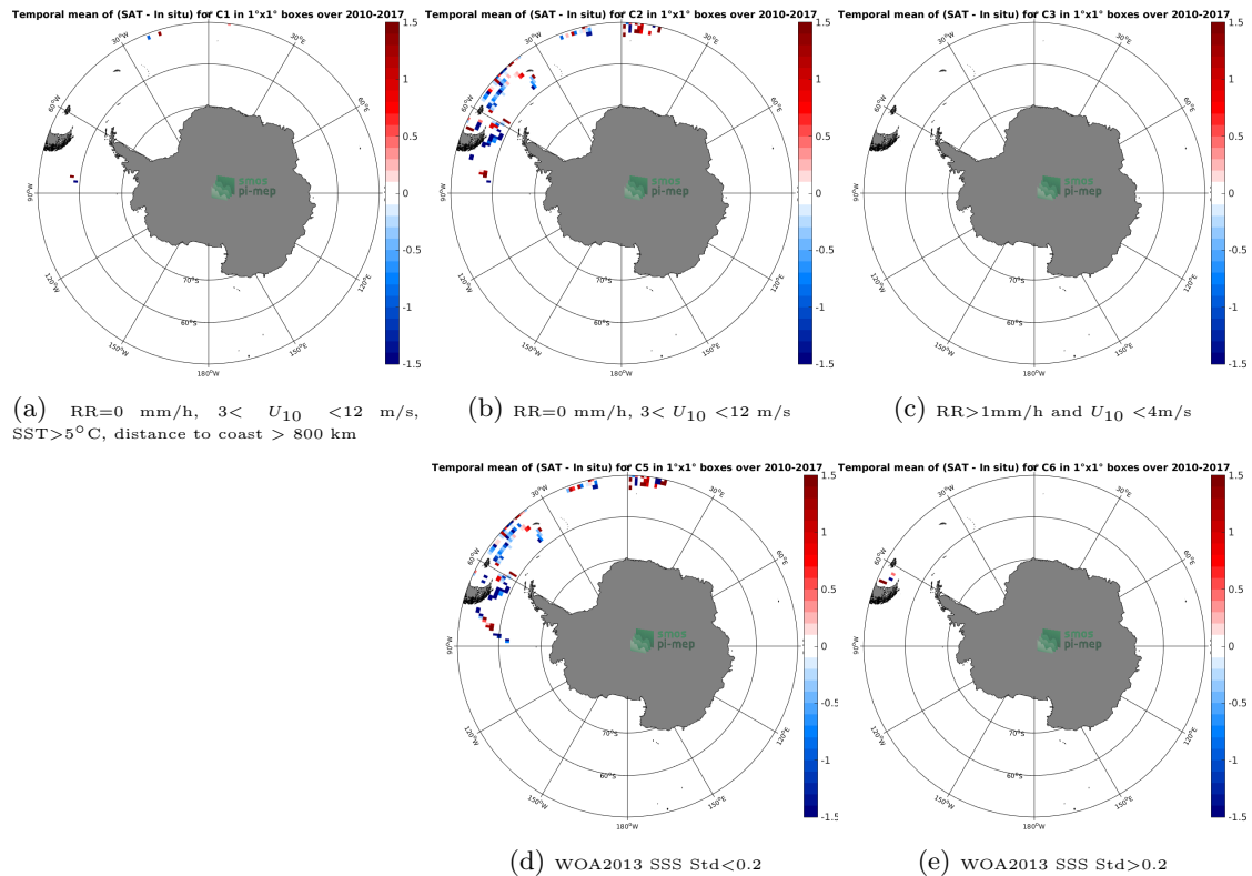
Figure 12: Temporal mean gridded over spatial boxes of size 1^\circ \times 1^\circ of \Delta SSS (SMOS-L2-DPGS-v662 - TSG-POLARSTERN) for 5 different subdatasets corresponding to:RR=0 mm/h, 3 < U_{10} < 12 m/s, SST >5^\circ C, distance to coast > 800 km (a), RR=0 mm/h, 3 < U_{10} < 12 m/s (b), RR >1 mm/h and U_{10} < 4 m/s (c), WOA2013 SSS Std <0.2 (d), WOA2013 SSS Std >0.2 (e).
