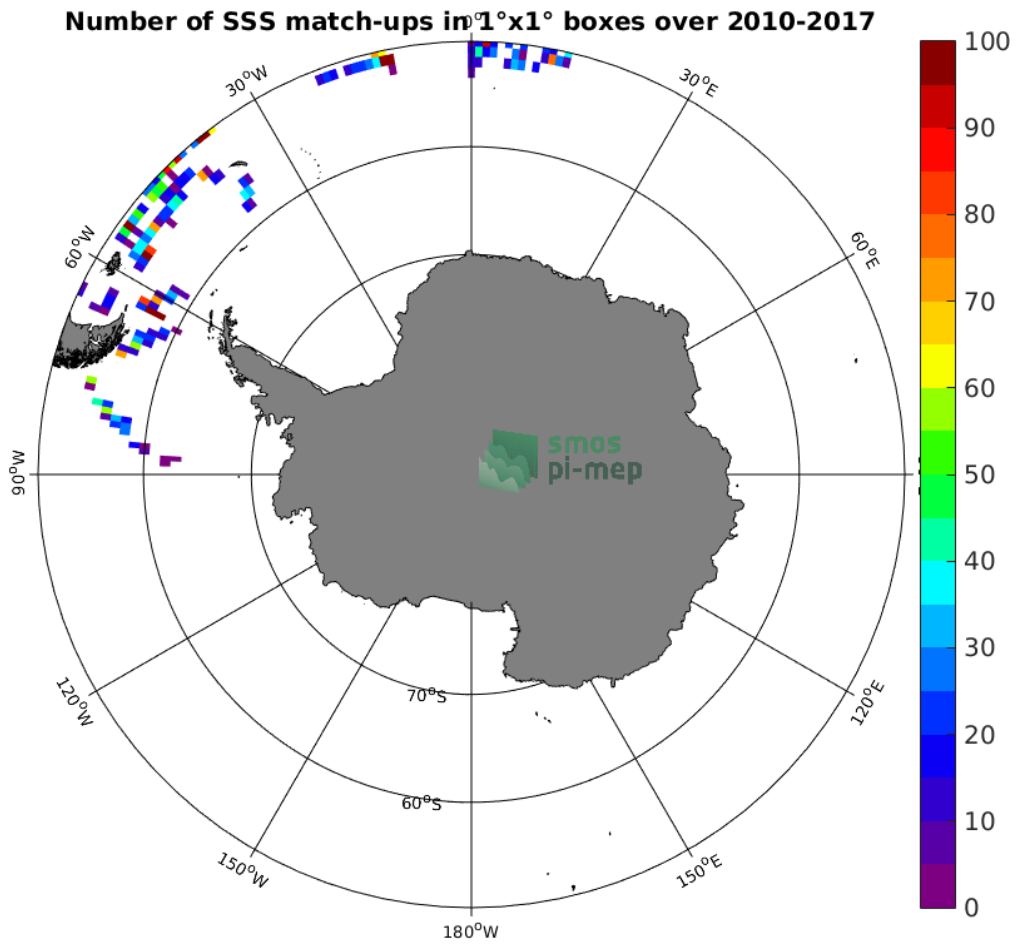
Figure 4: Number of SSS match-ups between TSG-POLARSTERN SSS and the SMOS-L2-DPGS-v662 SSS product for the Southern Ocean Pi-MEP region over 1°x1° boxes and for the full satellite product period.
