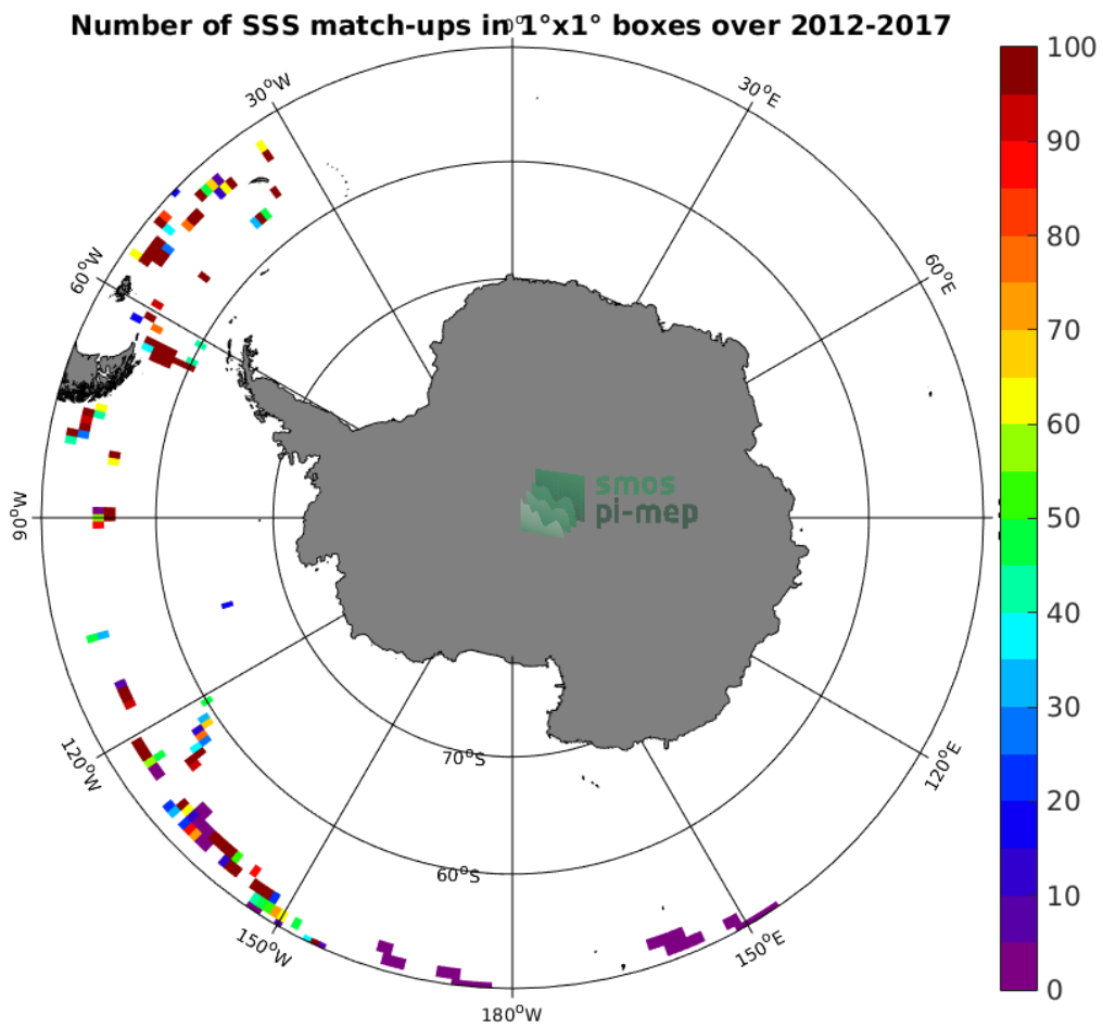
Figure 4: Number of SSS match-ups between TSG (GOSUD-Sailing-ship) SSS and the SMOS SSS L2 v662 (ESA) SSS product for the Southern Ocean Pi-MEP region over 1^\circ \times 1^\circ boxes and for the full satellite product period.
