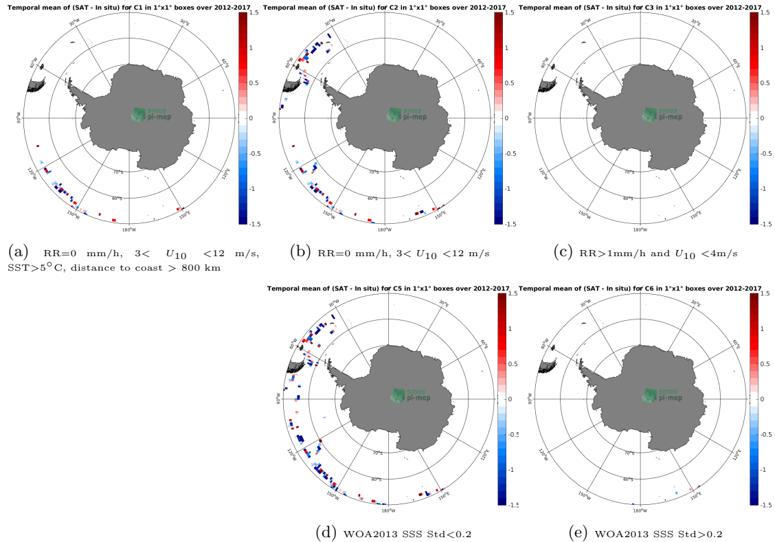
Figure 12: Temporal mean gridded over spatial boxes of size 1^\circ \times 1^\circ of \Delta SSS (SMOS SSS L2 v662 (ESA) - TSG (GOSUD-Sailing-ship)) for 5 different subdatasets corresponding to: RR=0 mm/h, 3 < U_{10} < 12 m/s, SST > 5^\circ\text{C} , distance to coast > 800 km (a), RR=0 mm/h, 3 < U_{10} < 12 m/s (b), RR > 1 mm/h and U_{10} < 4 m/s (c), WOA2013 SSS Std < 0.2 (d), WOA2013 SSS Std > 0.2 (e).
