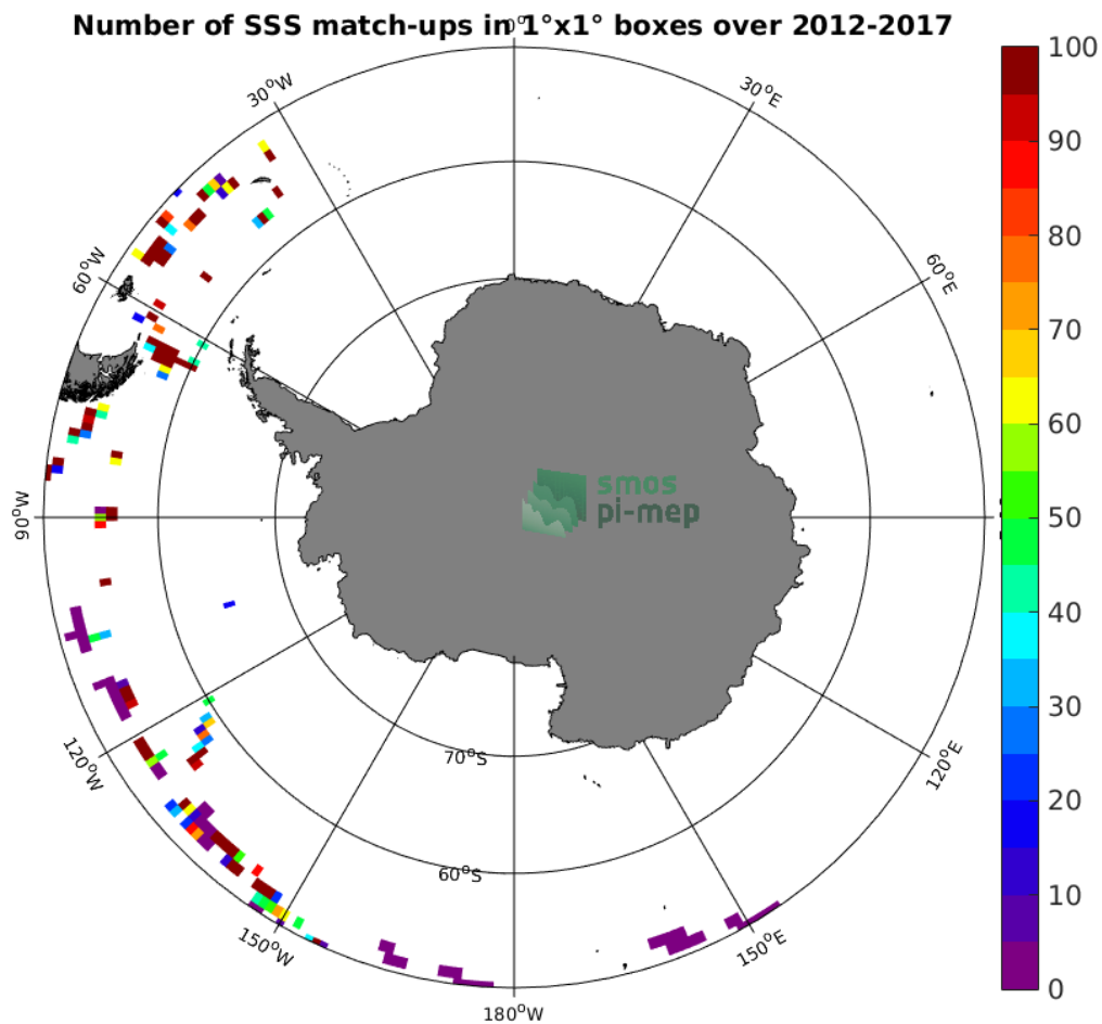
Figure 4: Number of SSS match-ups between TSG (GOSUD-Sailing-ship) SSS and the SMOS SSS L2 v662 (ESA) SSS product for the Southern Ocean Pi-MEP region over 1°x1° boxes and for the full satellite product period.
