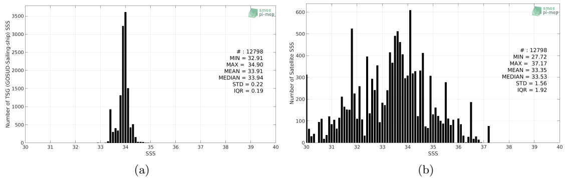
Figure 2: Histograms of SSS from TSG (GOSUD-Sailing-ship) (a) and SMOS SSS L2 v662 (ESA) (b) considering all match-up pairs per bins of 0.1 over the Southern Ocean Pi-MEP region and for the full satellite product period.
