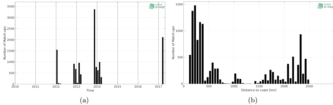
Figure 1: Number of match-ups between TSG (GOSUD-Sailing-ship) and SMOS SSS L2 v662 (ESA) SSS as a function of time (a) and as function of the distance to coast (b) over the Southern Ocean Pi-MEP region and for the full satellite product period.
