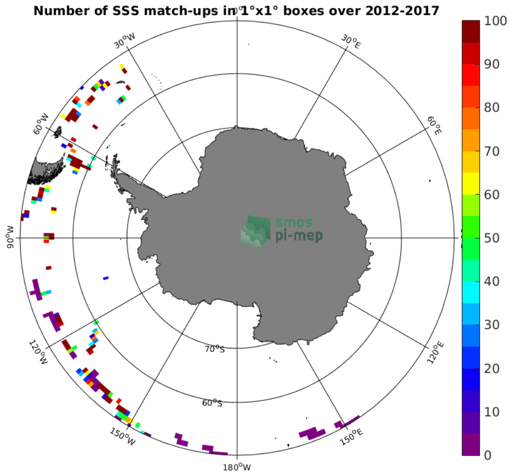
Figure 4: Number of SSS match-ups between TSG-GOSUD-Sailing-ship SSS and the SMOS L2 v662 (ESA) SSS product for the Southern Ocean Pi-MEP region over 1°x1° boxes and for the full satellite product period.
