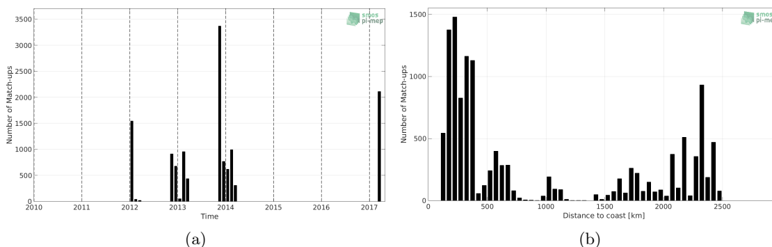
Figure 1: Number of match-ups between TSG-GOSUD-Sailing-ship and SMOS L2 v662 (ESA) SSS as a function of time (a) and as function of the distance to coast (b) over the Southern Ocean Pi-MEP region and for the full satellite product period.
