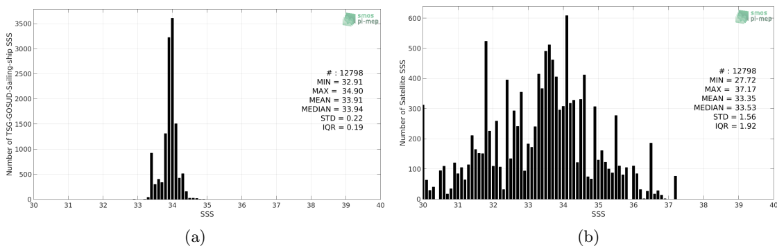
Figure 2: Histograms of SSS from TSG-GOSUD-Sailing-ship (a) and SMOS L2 v662 (ESA) (b) considering all match-up pairs per bins of 0.1 over the Southern Ocean Pi-MEP region and for the full satellite product period.
