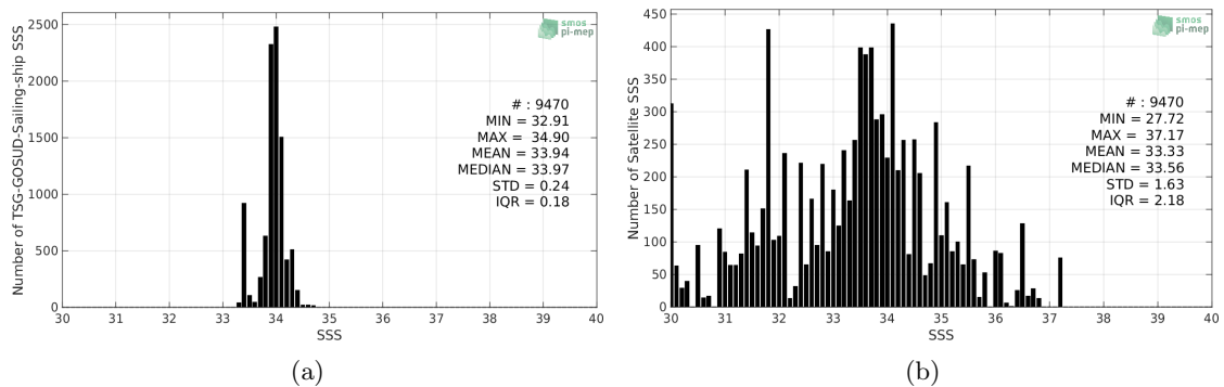
Figure 2: Histograms of SSS from TSG-GOSUD-Sailing-ship (a) and SMOS-L2-DPGS-v662 (b) considering all match-up pairs per bins of 0.1 over the Southern Ocean Pi-MEP region and for the full satellite product period.
