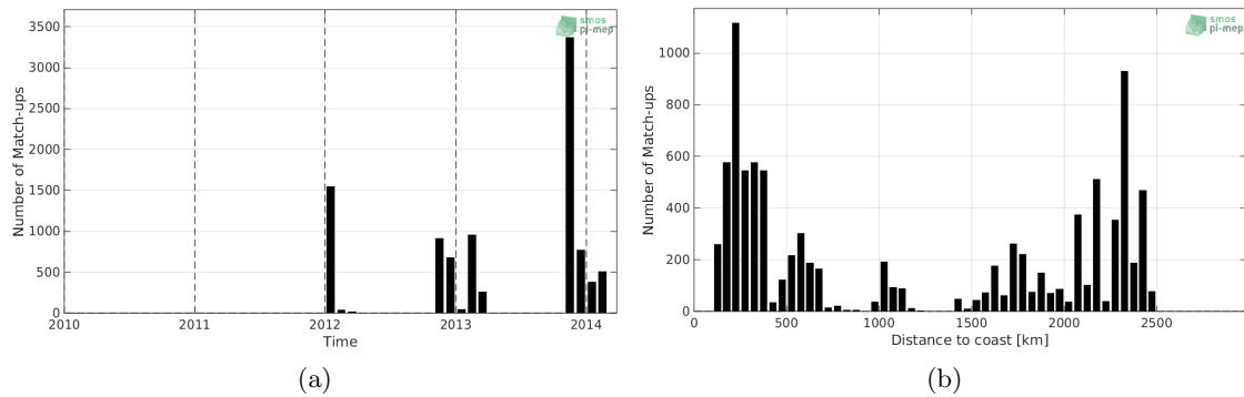
Figure 1: Number of match-ups between TSG-GOSUD-Sailing-ship and SMOS-L2-DPGS-v662 SSS as a function of time (a) and as function of the distance to coast (b) over the Southern Ocean Pi-MEP region and for the full satellite product period.
