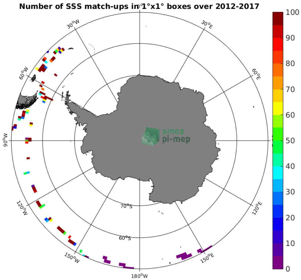
Figure 4: Number of SSS match-ups between TSG-GOSUD-Sailing-ship SSS and the SMOS-L2-DPGS-v662 SSS product for the Southern Ocean Pi-MEP region over 1°x1° boxes and for the full satellite product period.
