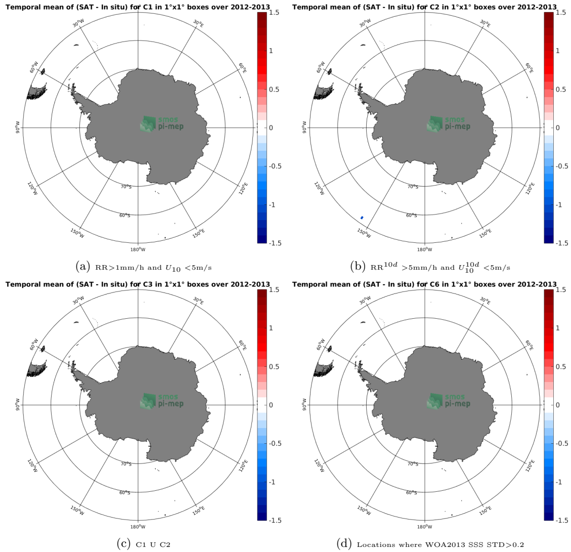
Figure 12: Temporal mean gridded over spatial boxes of size 1^\circ \times 1^\circ of \Delta SSS (SMOS-L2-DPGS-v662 - TSG-GOSUD-Sailing-ship) for 4 different subdatasets corresponding to: RR > 1mm/h and U_{10} < 5 m/s (a), RR^{10d} > 5 mm/h and U_{10}^{10d} < 5 m/s (b), C1 U C2 (c), Locations where WOA2013 SSS STD > 0.2 (d).
