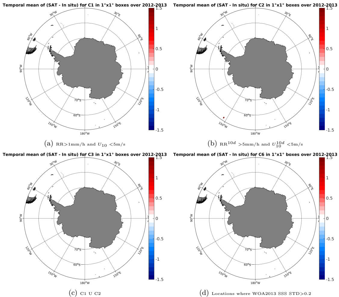
Figure 12: Temporal mean gridded over spatial boxes of size 1^\circ \times 1^\circ of \Delta SSS (SMOS-L2-DPGS-v662 - TSG-GOSUD-Sailing-ship) for 4 different subdatasets corresponding to: RR > 1\text{mm/h} and U_{10} < 5\text{m/s} (a), RR^{10d} > 5\text{mm/h} and U_{10}^{10d} < 5\text{m/s} (b), C1 U C2 (c), Locations where WOA2013 SSS STD > 0.2 (d).
