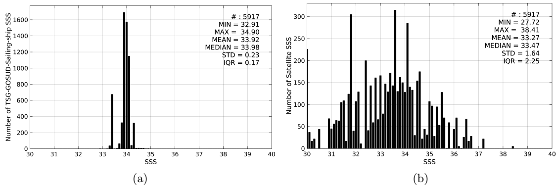
Figure 2: Histograms of SSS from TSG-GOSUD-Sailing-ship (a) and SMOS-L2-DPGS-v662 (b) considering all match-up pairs per bins of 0.1 over the Southern Ocean Pi-MEP region and for the full satellite product period.
