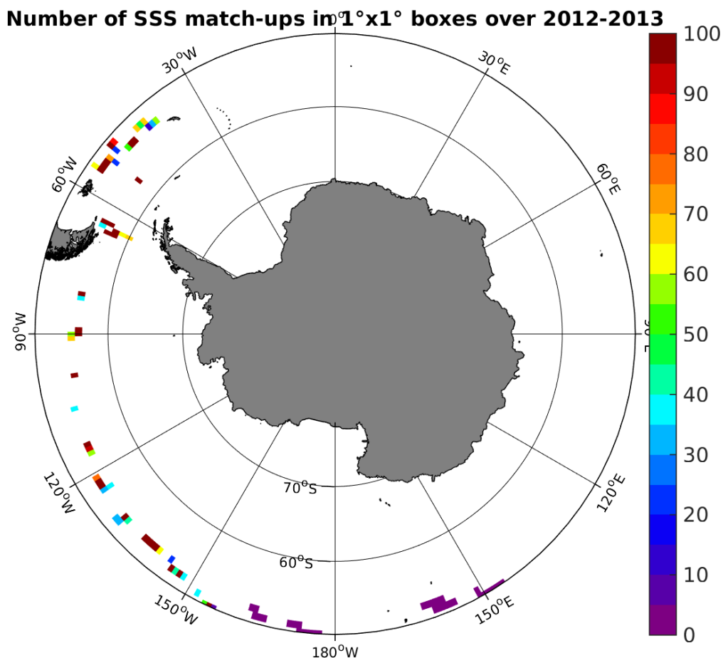
Figure 4: Number of SSS match-ups between TSG-GOSUD-Sailing-ship SSS and the SMOS-L2-DPGS-v662 SSS product for the Southern Ocean Pi-MEP region over 1°x1° boxes and for the full satellite product period.
