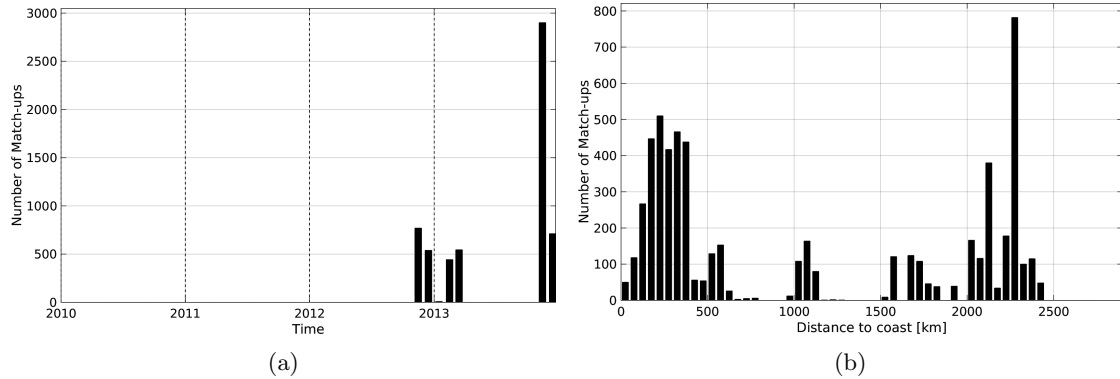
Figure 1: Number of match-ups between TSG-GOSUD-Sailing-ship and SMOS-L2-DPGS-v662 SSS as a function of time (a) and as function of the distance to coast (b) over the Southern Ocean Pi-MEP region and for the full satellite product period.
