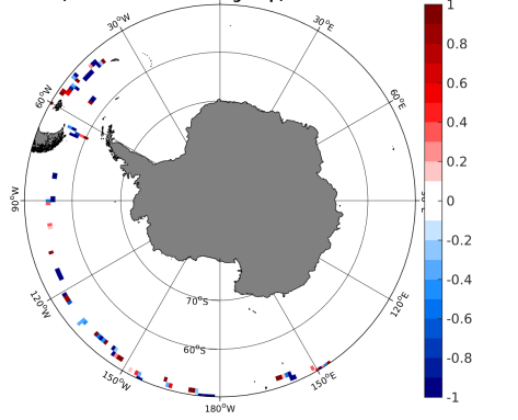
(e) MEAN( \Delta SSS) (Satellite - TSG-GOSUD-Sailing-ship)
