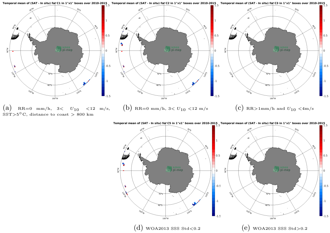
Figure 12: Temporal mean gridded over spatial boxes of size 1°x1° of \Delta SSS (SMOS SSS L2 v662 (ESA) - TSG (GOSUD-Research-vessel)) for 5 different subdatasets corresponding to: RR=0 mm/h, 3 < U_{10} < 12 m/s, SST > 5°C, distance to coast > 800 km (a), RR=0 mm/h, 3 < U_{10} < 12 m/s (b), RR > 1mm/h and U_{10} < 4 m/s (c), WOA2013 SSS Std < 0.2 (d), WOA2013 SSS Std > 0.2 (e).
