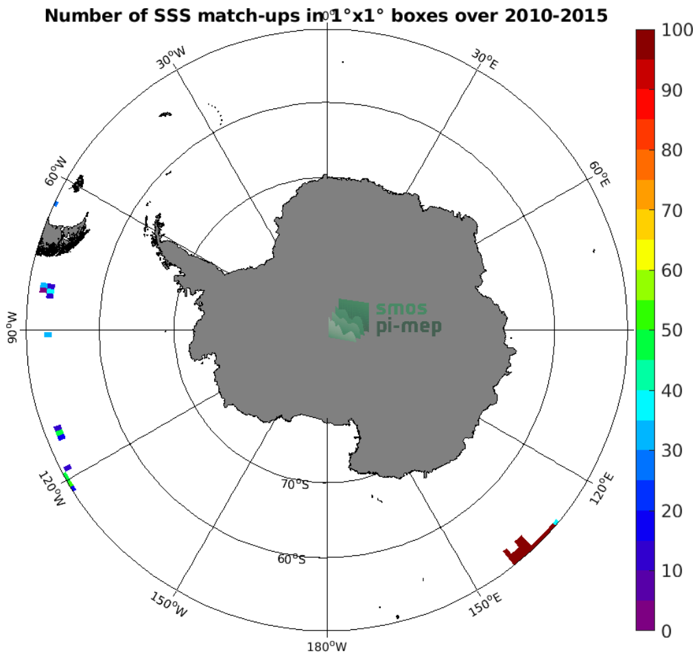
Figure 4: Number of SSS match-ups between TSG (GOSUD-Research-vessel) SSS and the SMOS SSS L2 v662 (ESA) SSS product for the Southern Ocean Pi-MEP region over 1^\circ \times 1^\circ boxes and for the full satellite product period.
