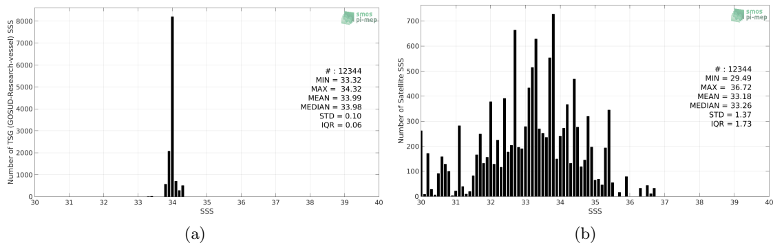
Figure 2: Histograms of SSS from TSG (GOSUD-Research-vessel) (a) and SMOS SSS L2 v662 (ESA) (b) considering all match-up pairs per bins of 0.1 over the Southern Ocean Pi-MEP region and for the full satellite product period.
