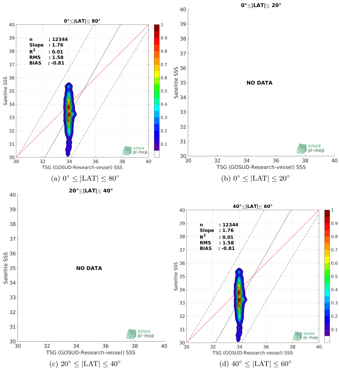
Figure 9: Contour maps of the concentration of SMOS SSS L2 v662 (ESA) SSS (y-axis) versus TSG (GOSUD-Research-vessel) SSS (x-axis) at match-up pairs for different latitude bands. For each plot, the red line shows x=y . The black thin and dashed lines indicate a linear fit through the data cloud and the \pm 95\% confidence levels, respectively. The number match-up pairs n , the slope and R^2 coefficient of the linear fit, the root mean square (RMS) and the mean bias between satellite and in situ data are indicated for each latitude band in each plots.
