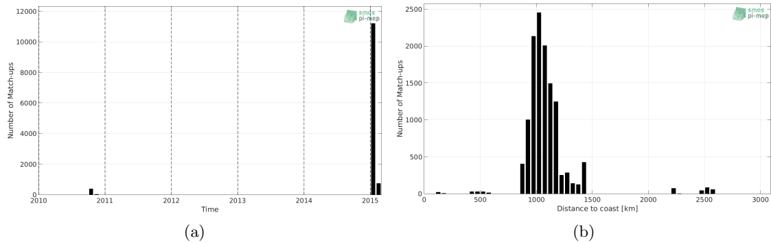
Figure 1: Number of match-ups between TSG (GOSUD-Research-vessel) and SMOS SSS L2 v662 (ESA) SSS as a function of time (a) and as function of the distance to coast (b) over the Southern Ocean Pi-MEP region and for the full satellite product period.
