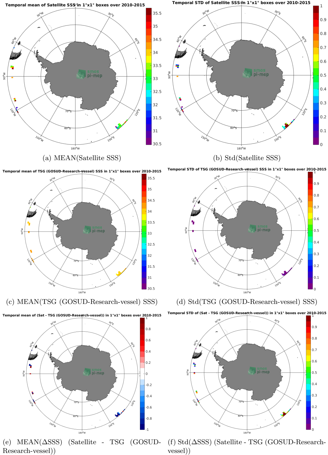
Figure 6: Temporal mean (left) and Std (right) of SSS from SMOS SSS L2 v662 (ESA) (top), TSG (GOSUD-Research-vessel) (middle), and of \Delta SSS (Satellite - TSG (GOSUD-Research-vessel)). Only match-up pairs are used to generate these maps.
