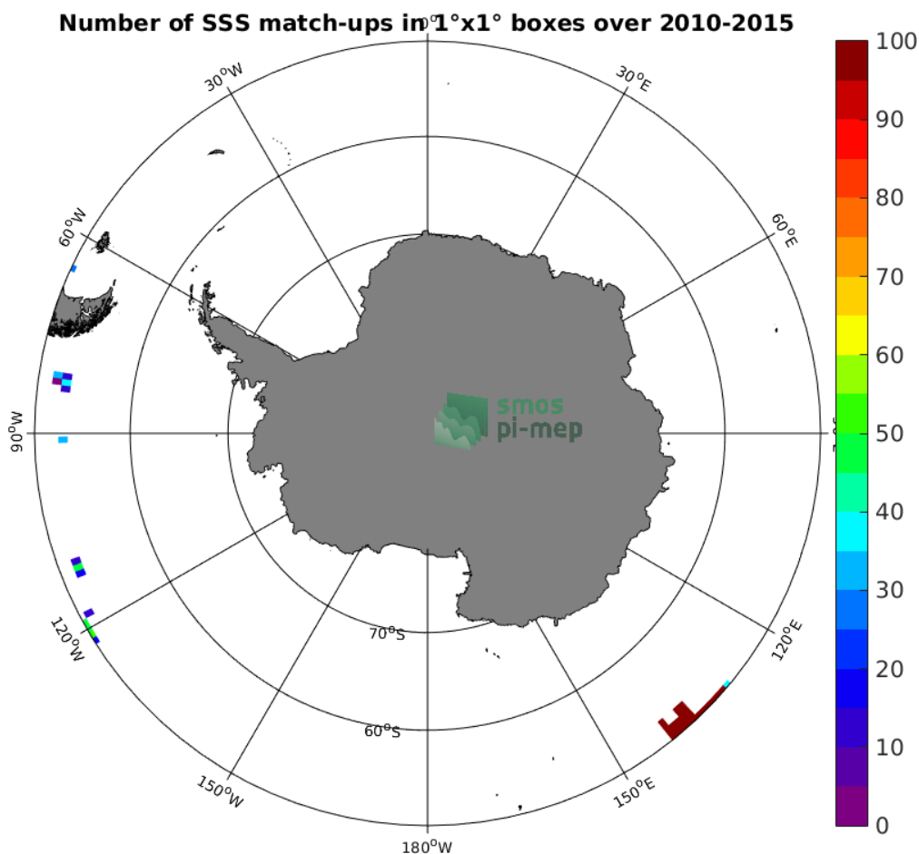
Figure 4: Number of SSS match-ups between TSG (GOSUD-Research-vessel) SSS and the SMOS SSS L2 v662 (ESA) SSS product for the Southern Ocean Pi-MEP region over 1°x1° boxes and for the full satellite product period.
