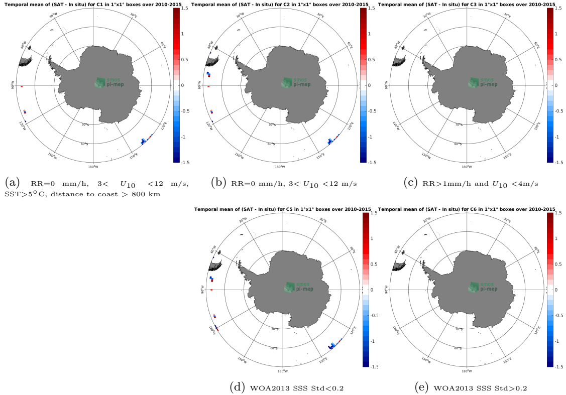
Figure 12: Temporal mean gridded over spatial boxes of size 1°x1° of \Delta SSS (SMOS SSS L2 v662 (ESA) - TSG (GOSUD-Research-vessel)) for 5 different subdatasets corresponding to:RR=0 mm/h, 3 < U_{10} < 12 m/s, SST>5°C, distance to coast > 800 km (a), RR=0 mm/h, 3 < U_{10} < 12 m/s (b), RR>1mm/h and U_{10} < 4 m/s (c), WOA2013 SSS Std<0.2 (d), WOA2013 SSS Std>0.2 (e).
