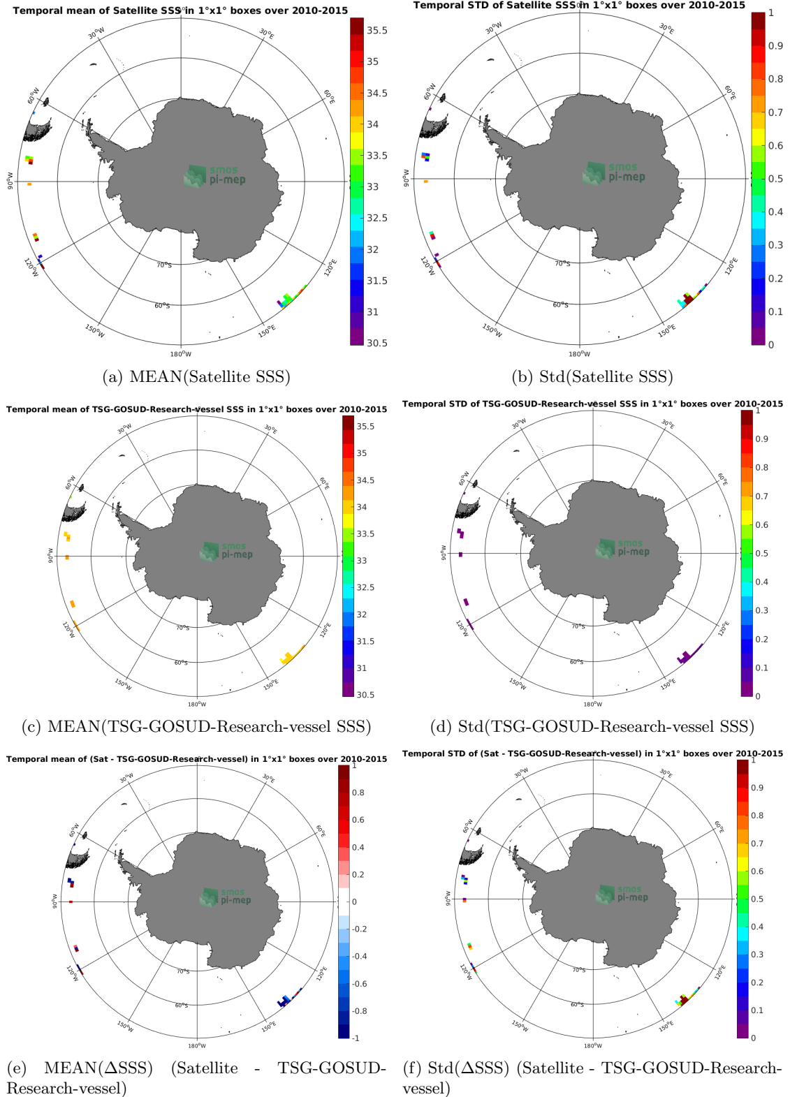
Figure 6: Temporal mean (left) and Std (right) of SSS from SMOS L2 v662 (ESA) (top), TSG-GOSUD-Research-vessel (middle), and of \Delta SSS (Satellite - TSG-GOSUD-Research-vessel). Only match-up pairs are used to generate these maps.
