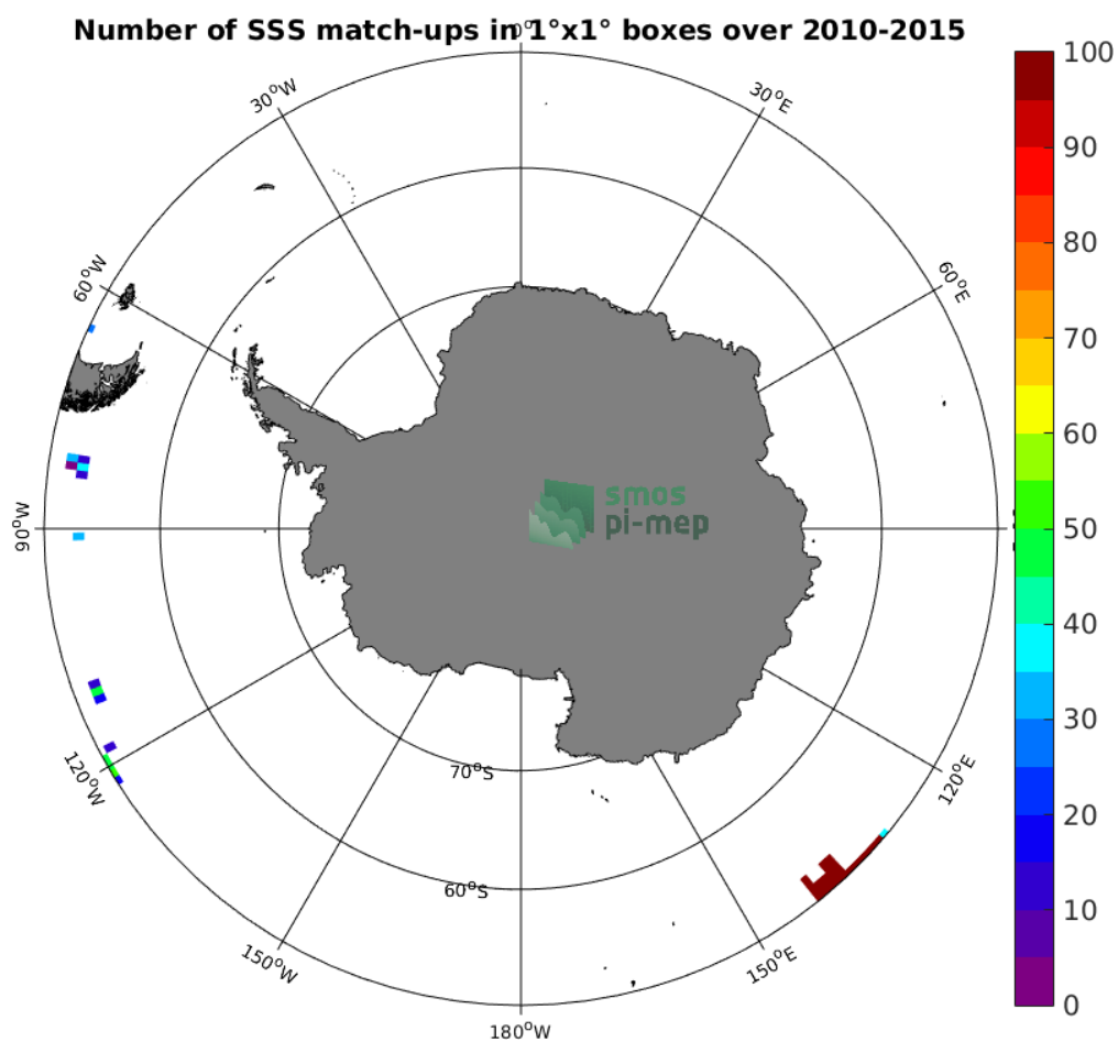
Figure 4: Number of SSS match-ups between TSG-GOSUD-Research-vessel SSS and the SMOS L2 v662 (ESA) SSS product for the Southern Ocean Pi-MEP region over 1°x1° boxes and for the full satellite product period.
