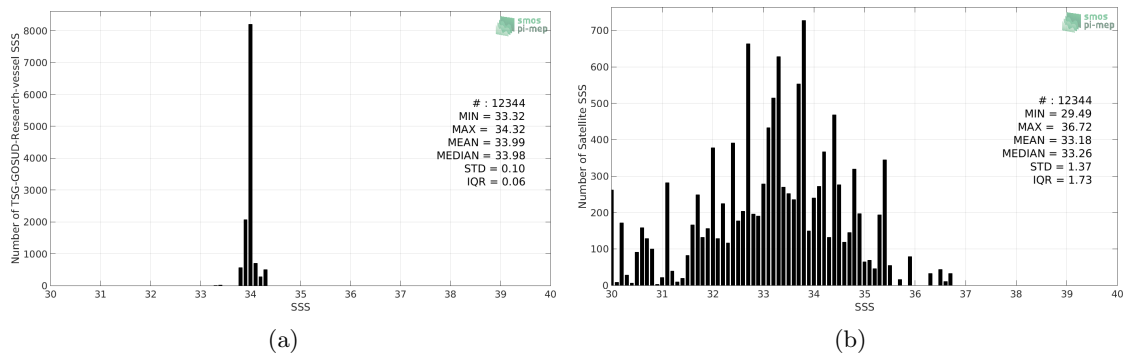
Figure 2: Histograms of SSS from TSG-GOSUD-Research-vessel (a) and SMOS L2 v662 (ESA) (b) considering all match-up pairs per bins of 0.1 over the Southern Ocean Pi-MEP region and for the full satellite product period.
