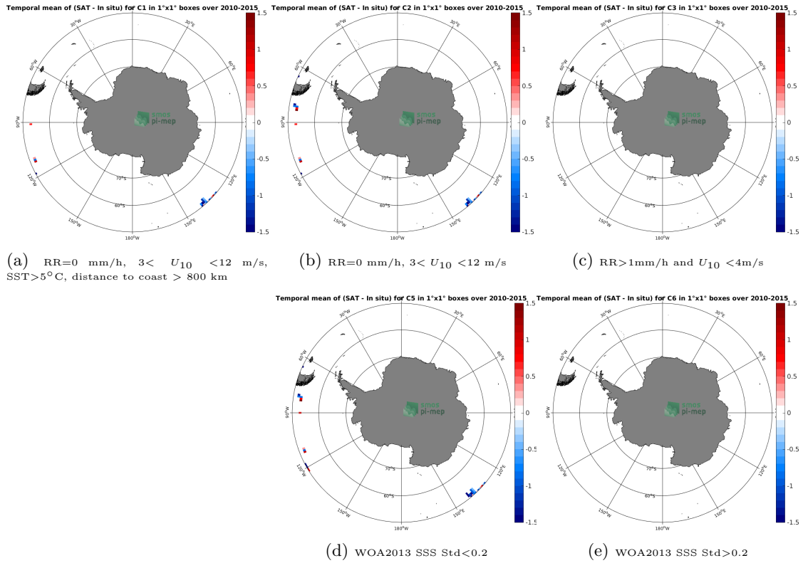
Figure 12: Temporal mean gridded over spatial boxes of size 1°x1° of \Delta SSS (SMOS L2 v662 (ESA) - TSG-GOSUD-Research-vessel) for 5 different subdatasets corresponding to: RR=0 mm/h, 3 < U_{10} < 12 m/s, SST > 5°C, distance to coast > 800 km (a), RR=0 mm/h, 3 < U_{10} < 12 m/s (b), RR > 1mm/h and U_{10} < 4 m/s (c), WOA2013 SSS Std < 0.2 (d), WOA2013 SSS Std > 0.2 (e).
