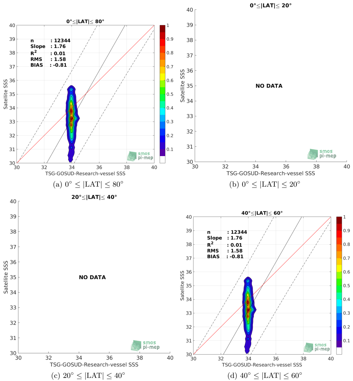
Figure 9: Contour maps of the concentration of SMOS L2 v662 (ESA) SSS (y-axis) versus TSG-GOSUD-Research-vessel SSS (x-axis) at match-up pairs for different latitude bands. For each plot, the red line shows x=y . The black thin and dashed lines indicate a linear fit through the data cloud and the \pm 95\% confidence levels, respectively. The number match-up pairs n , the slope and R^2 coefficient of the linear fit, the root mean square (RMS) and the mean bias between satellite and in situ data are indicated for each latitude band in each plots.
