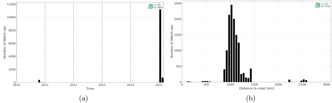
Figure 1: Number of match-ups between TSG-GOSUD-Research-vessel and SMOS L2 v662 (ESA) SSS as a function of time (a) and as function of the distance to coast (b) over the Southern Ocean Pi-MEP region and for the full satellite product period.
