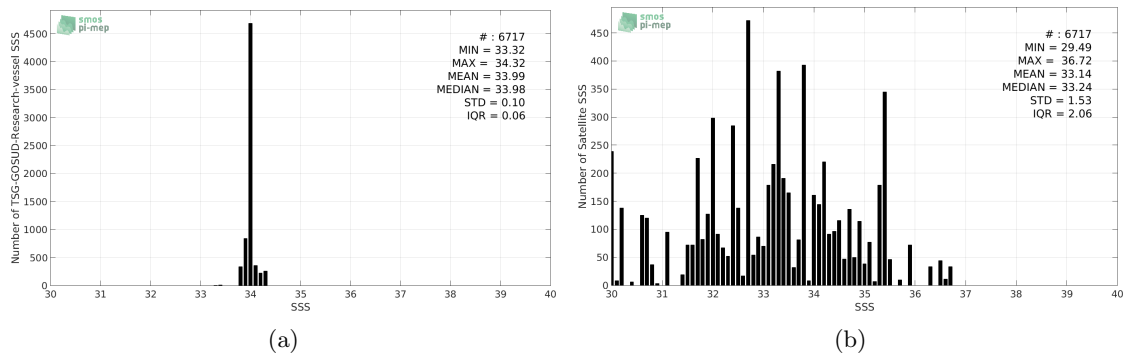
Figure 2: Histograms of SSS from TSG-GOSUD-Research-vessel (a) and SMOS-L2-DPGS-v662 (b) considering all match-up pairs per bins of 0.1 over the Southern Ocean Pi-MEP region and for the full satellite product period.
