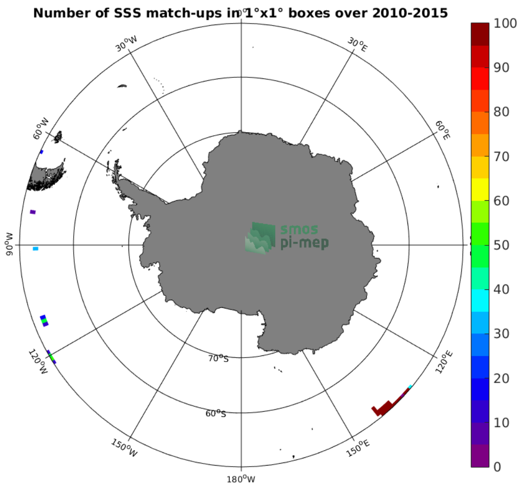
Figure 4: Number of SSS match-ups between TSG-GOSUD-Research-vessel SSS and the SMOS-L2-DPGS-v662 SSS product for the Southern Ocean Pi-MEP region over 1°x1° boxes and for the full satellite product period.
