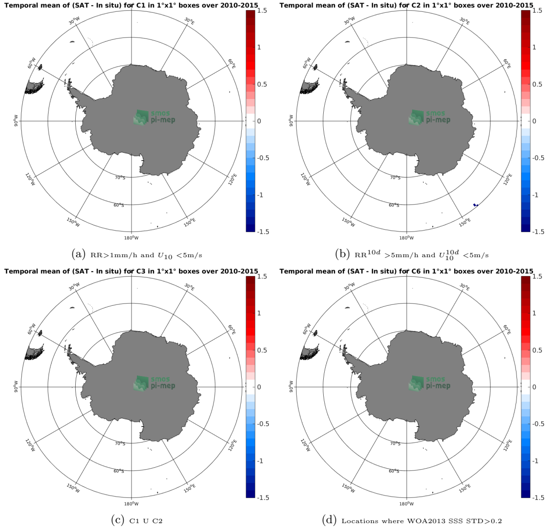
Figure 12: Temporal mean gridded over spatial boxes of size 1^\circ \times 1^\circ of \Delta SSS (SMOS-L2-DPGS-v662 - TSG-GOSUD-Research-vessel) for 4 different subdatasets corresponding to: RR > 1mm/h and U_{10} < 5\text{m/s} (a), RR^{10d} > 5\text{mm/h} and U_{10}^{10d} < 5\text{m/s} (b), C1 U C2 (c), Locations where WOA2013 SSS STD > 0.2 (d).
