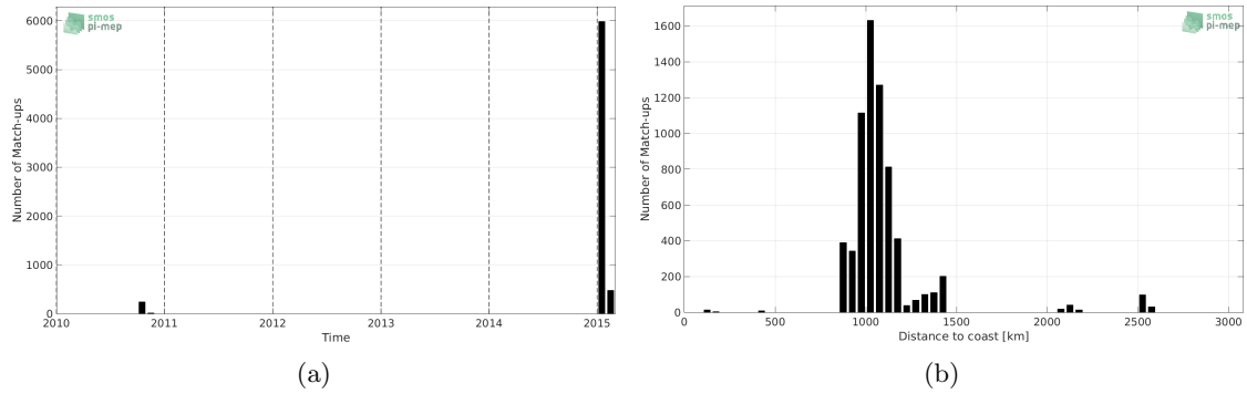
Figure 1: Number of match-ups between TSG-GOSUD-Research-vessel and SMOS-L2-DPGS-v662 SSS as a function of time (a) and as function of the distance to coast (b) over the Southern Ocean Pi-MEP region and for the full satellite product period.
