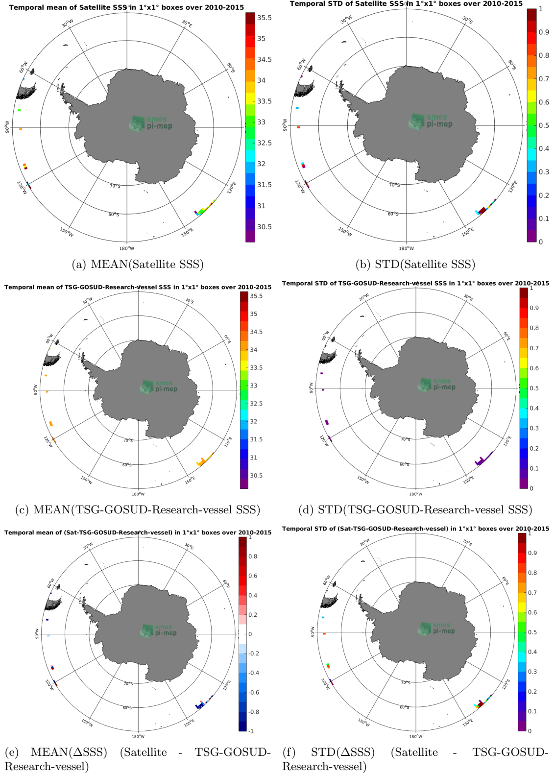
Figure 6: Temporal mean (left) and STD (right) of SSS from SMOS-L2-DPGS-v662 (top), TSG-GOSUD-Research-vessel (middle), and of \Delta SSS 2 (Satellite - TSG-GOSUD-Research-vessel). Only match-up pairs are used to generate these maps.
