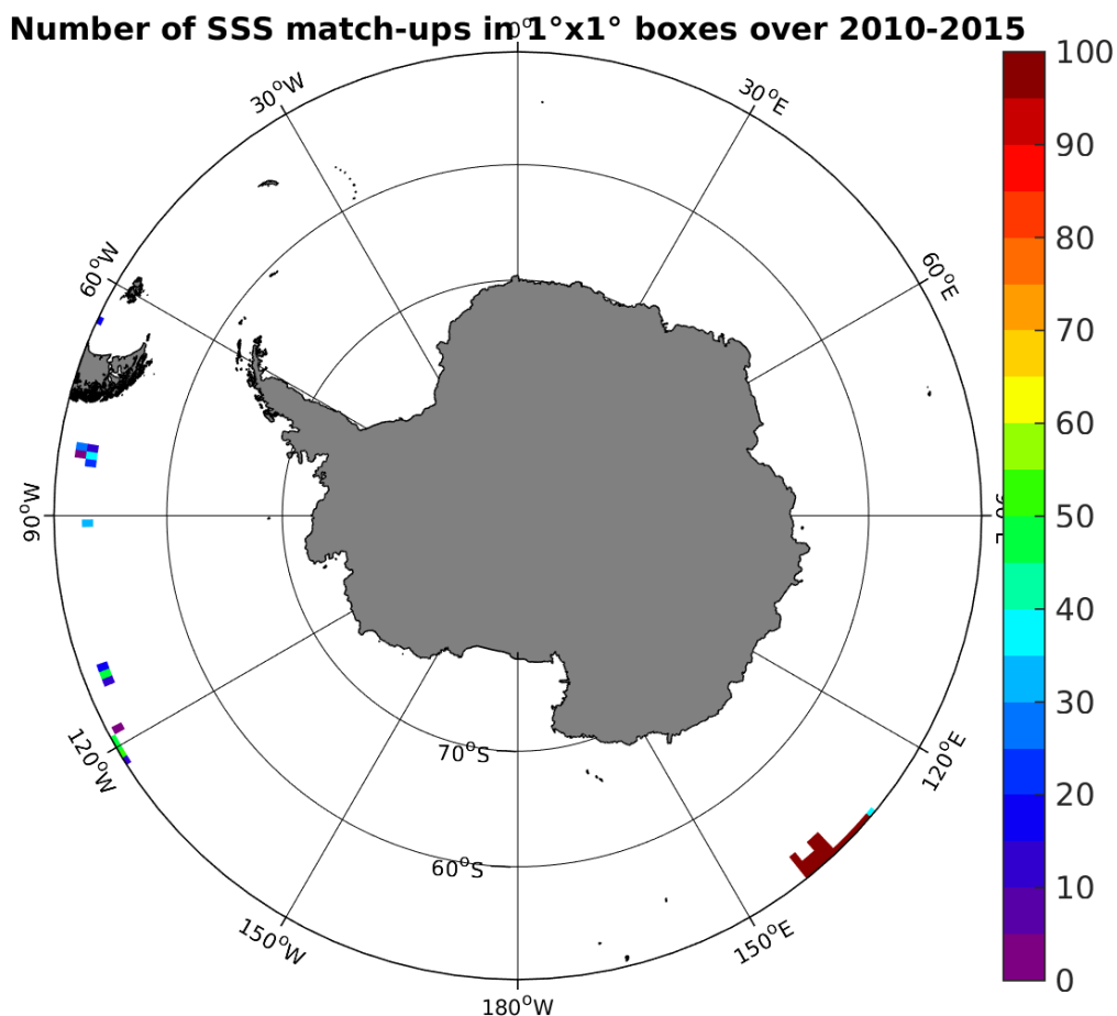
Figure 4: Number of SSS match-ups between TSG-GOSUD-Research-vessel SSS and the SMOS-L2-DPGS-v662 SSS product for the Southern Ocean Pi-MEP region over 1°x1° boxes and for the full satellite product period.
