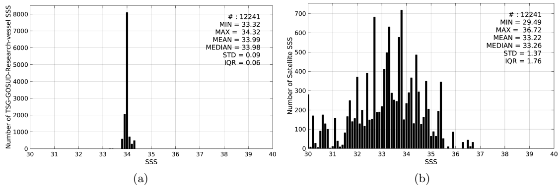
Figure 2: Histograms of SSS from TSG-GOSUD-Research-vessel (a) and SMOS-L2-DPGS-v662 (b) considering all match-up pairs per bins of 0.1 over the Southern Ocean Pi-MEP region and for the full satellite product period.
