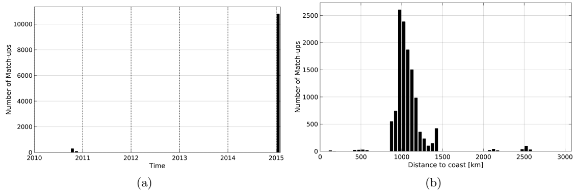
Figure 1: Number of match-ups between TSG-GOSUD-Research-vessel and SMOS-L2-DPGS-v662 SSS as a function of time (a) and as function of the distance to coast (b) over the Southern Ocean Pi-MEP region and for the full satellite product period.
