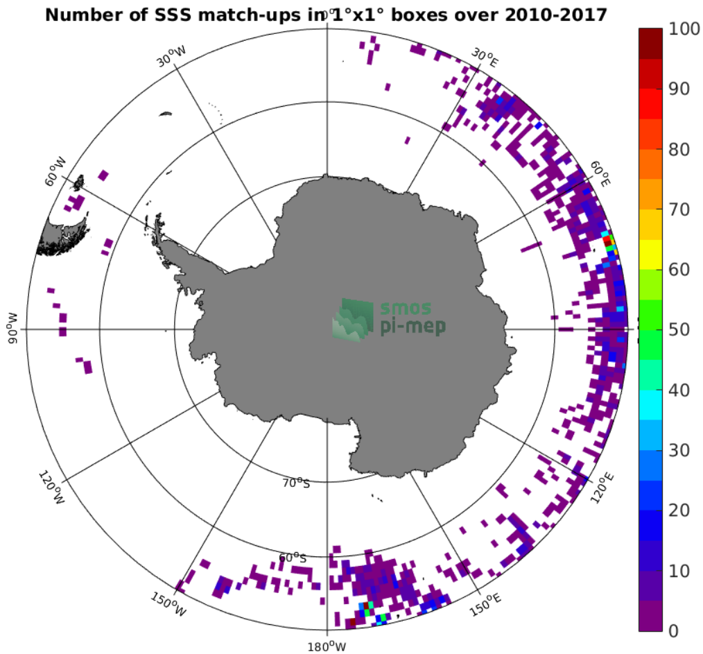
Figure 4: Number of SSS match-ups between Sea mammals SSS and the SMOS SSS L2 v662 (ESA) SSS product for the Southern Ocean Pi-MEP region over 1^\circ \times 1^\circ boxes and for the full satellite product period.
