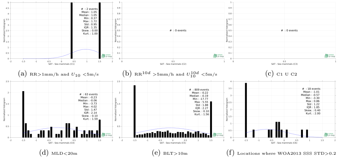
Figure 13: Normalized histogram of \Delta SSS (SMOS-L2-DPGS-v662 - Sea mammals) for 6 different subdatasets corresponding to: RR > 1\text{mm/h} and U_{10} < 5\text{m/s} (a), RR^{10d} > 5\text{mm/h} and U_{10}^{10d} < 5\text{m/s} (b), C1 U C2 (c), MLD < 20\text{m} (d), BLT > 10\text{m} (e), Locations where WOA2013 SSS STD > 0.2 (f).
