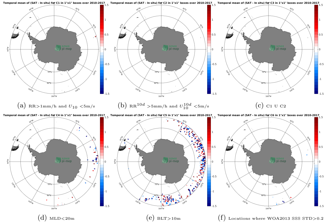
Figure 12: Temporal mean gridded over spatial boxes of size 1^\circ \times 1^\circ of \Delta\text{SSS} (SMOS-L2-DPGS-v662 - Sea mammals) for 6 different subdatasets corresponding to: \text{RR} > 1\text{mm/h} and U_{10} < 5\text{m/s} (a), \text{RR}^{10d} > 5\text{mm/h} and U_{10}^{10d} < 5\text{m/s} (b), C1 U C2 (c), \text{MLD} < 20\text{m} (d), \text{BLT} > 10\text{m} (e), Locations where WOA2013 SSS STD > 0.2 (f).
