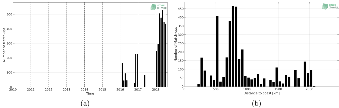
Figure 1: Number of match-ups between Surface drifters and SMOS SSS L2 v662 (ESA) SSS as a function of time (a) and as function of the distance to coast (b) over the Southern Ocean Pi-MEP region and for the full satellite product period.
