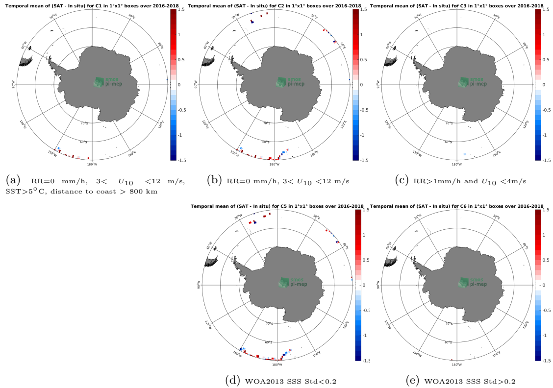
Figure 11: Temporal mean gridded over spatial boxes of size 1^{\circ}\times 1^{\circ} of \Delta\text{SSS} (SMOS SSS L2 v662 (ESA) - Surface drifters) for 5 different subdatasets corresponding to:RR=0 mm/h, 3 < U_{10} < 12 m/s, SST >5^{\circ}\text{C} , distance to coast > 800 km (a), RR=0 mm/h, 3 < U_{10} < 12 m/s (b), RR >1 mm/h and U_{10} < 4 m/s (c), WOA2013 SSS Std <0.2 (d), WOA2013 SSS Std >0.2 (e).
