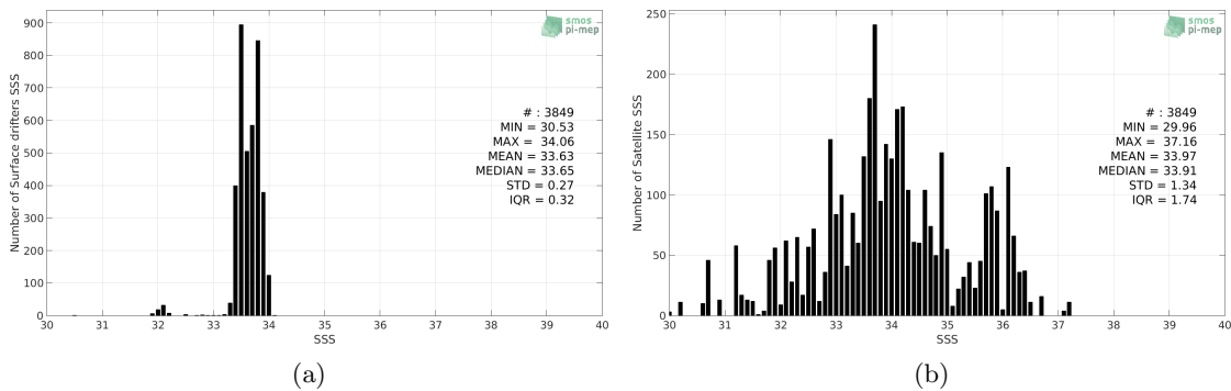
Figure 2: Histograms of SSS from Surface drifters (a) and SMOS SSS L2 v662 (ESA) (b) considering all match-up pairs per bins of 0.1 over the Southern Ocean Pi-MEP region and for the full satellite product period.
