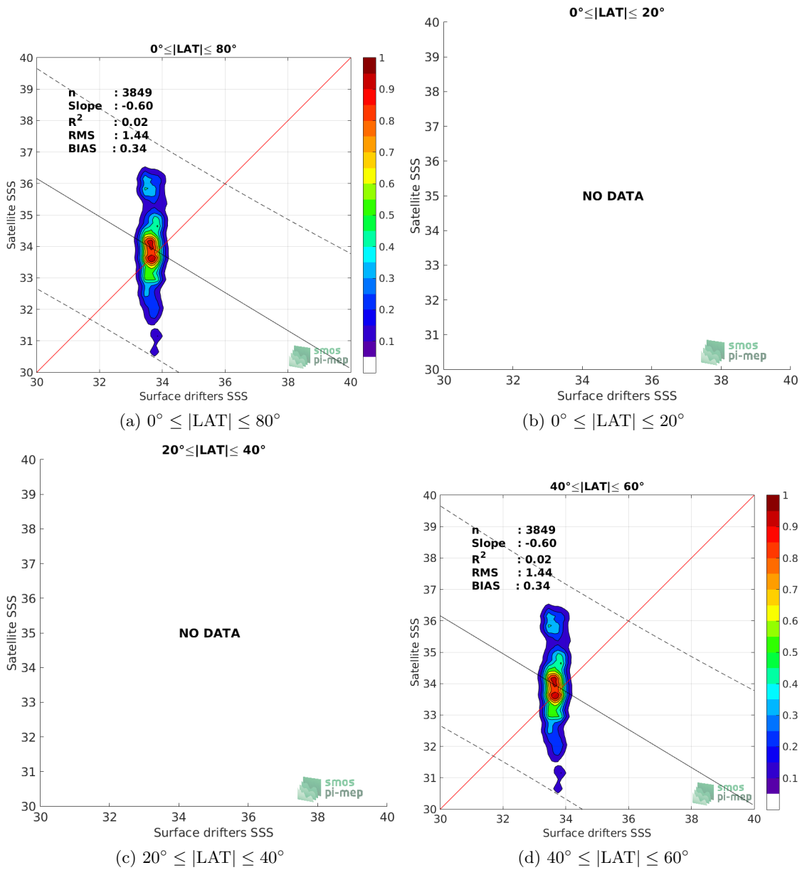
Figure 8: Contour maps of the concentration of SMOS SSS L2 v662 (ESA) SSS (y-axis) versus Surface drifters SSS (x-axis) at match-up pairs for different latitude bands. For each plot, the red line shows x=y . The black thin and dashed lines indicate a linear fit through the data cloud and the \pm 95\% confidence levels, respectively. The number match-up pairs n , the slope and R^2 coefficient of the linear fit, the root mean square (RMS) and the mean bias between satellite and in situ data are indicated for each latitude band in each plots.
