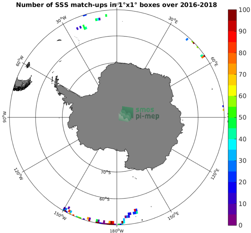
Figure 3: Number of SSS match-ups between Surface drifters SSS and the SMOS SSS L2 v662 (ESA) SSS product for the Southern Ocean Pi-MEP region over 1^\circ \times 1^\circ boxes and for the full satellite product period.
