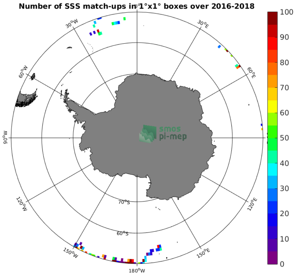
Figure 3: Number of SSS match-ups between Surface drifters SSS and the SMOS SSS L2 v662 (ESA) SSS product for the Southern Ocean Pi-MEP region over 1^\circ \times 1^\circ boxes and for the full satellite product period.
