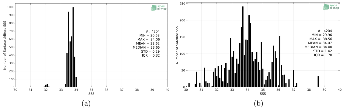
Figure 2: Histograms of SSS from Surface drifters (a) and SMOS L2 v662 (ESA) (b) considering all match-up pairs per bins of 0.1 over the Southern Ocean Pi-MEP region and for the full satellite product period.
