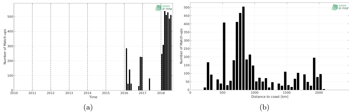
Figure 1: Number of match-ups between Surface drifters and SMOS L2 v662 (ESA) SSS as a function of time (a) and as function of the distance to coast (b) over the Southern Ocean Pi-MEP region and for the full satellite product period.
