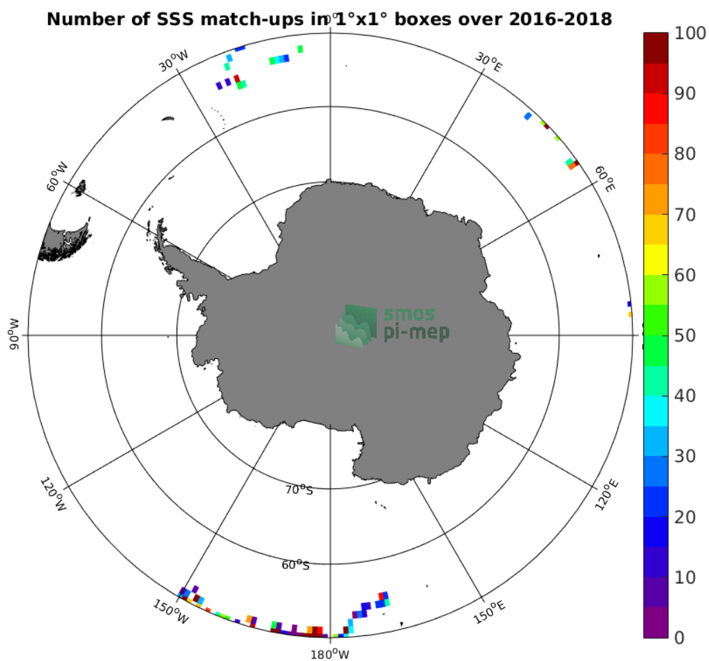
Figure 3: Number of SSS match-ups between Surface drifters SSS and the SMOS L2 v662 (ESA) SSS product for the Southern Ocean Pi-MEP region over 1^\circ \times 1^\circ boxes and for the full satellite product period.
