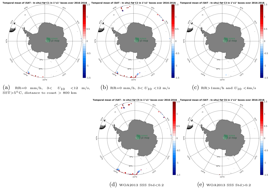
Figure 11: Temporal mean gridded over spatial boxes of size 1^{\circ}\times 1^{\circ} of \Delta\text{SSS} (SMOS L2 v662 (ESA) - Surface drifters) for 5 different subdatasets corresponding to: \text{RR}=0 mm/h, 3 < U_{10} < 12 m/s, \text{SST}>5^{\circ}\text{C} , distance to coast > 800 km (a), \text{RR}=0 mm/h, 3 < U_{10} < 12 m/s (b), \text{RR}>1 mm/h and U_{10} < 4 m/s (c), WOA2013 SSS Std < 0.2 (d), WOA2013 SSS Std > 0.2 (e).
