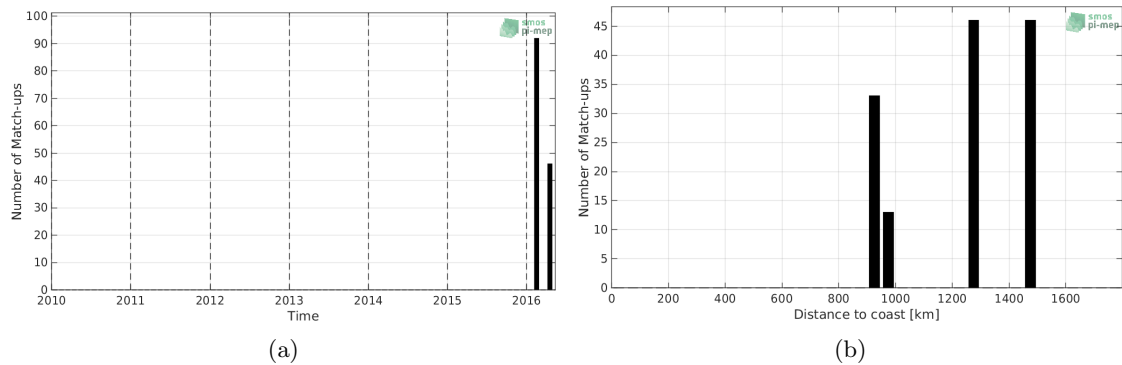
Figure 1: Number of match-ups between Surface drifters and SMOS-L2-DPGS-v662 SSS as a function of time (a) and as function of the distance to coast (b) over the Southern Ocean Pi-MEP region and for the full satellite product period.
