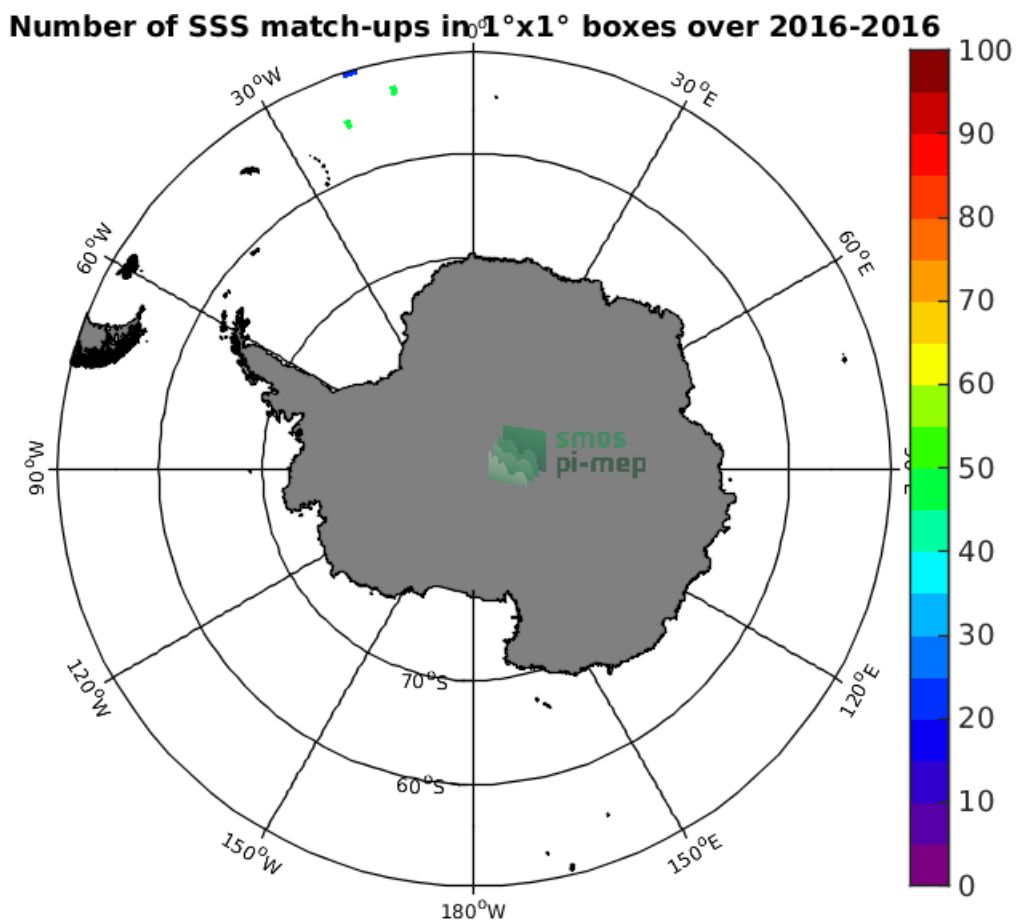
Figure 3: Number of SSS match-ups between Surface drifters SSS and the SMOS-L2-DPGS-v662 SSS product for the Southern Ocean Pi-MEP region over 1^\circ \times 1^\circ boxes and for the full satellite product period.
