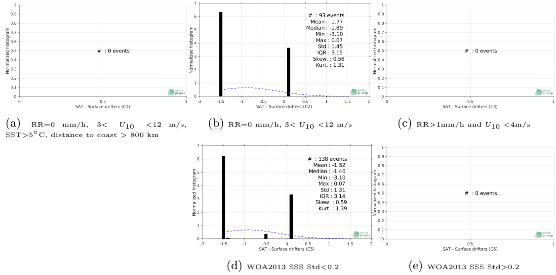
Figure 12: Normalized histogram of \Delta\text{SSS} (SMOS-L2-DPGS-v662 - Surface drifters) for 5 different subdatasets corresponding to: RR=0 mm/h, 3 < U_{10} < 12 m/s, SST > 5^\circ\text{C} , distance to coast > 800 km (a), RR=0 mm/h, 3 < U_{10} < 12 m/s (b), RR > 1\text{mm/h} and U_{10} < 4\text{m/s} (c), WOA2013 SSS Std < 0.2 (d), WOA2013 SSS Std > 0.2 (e).
