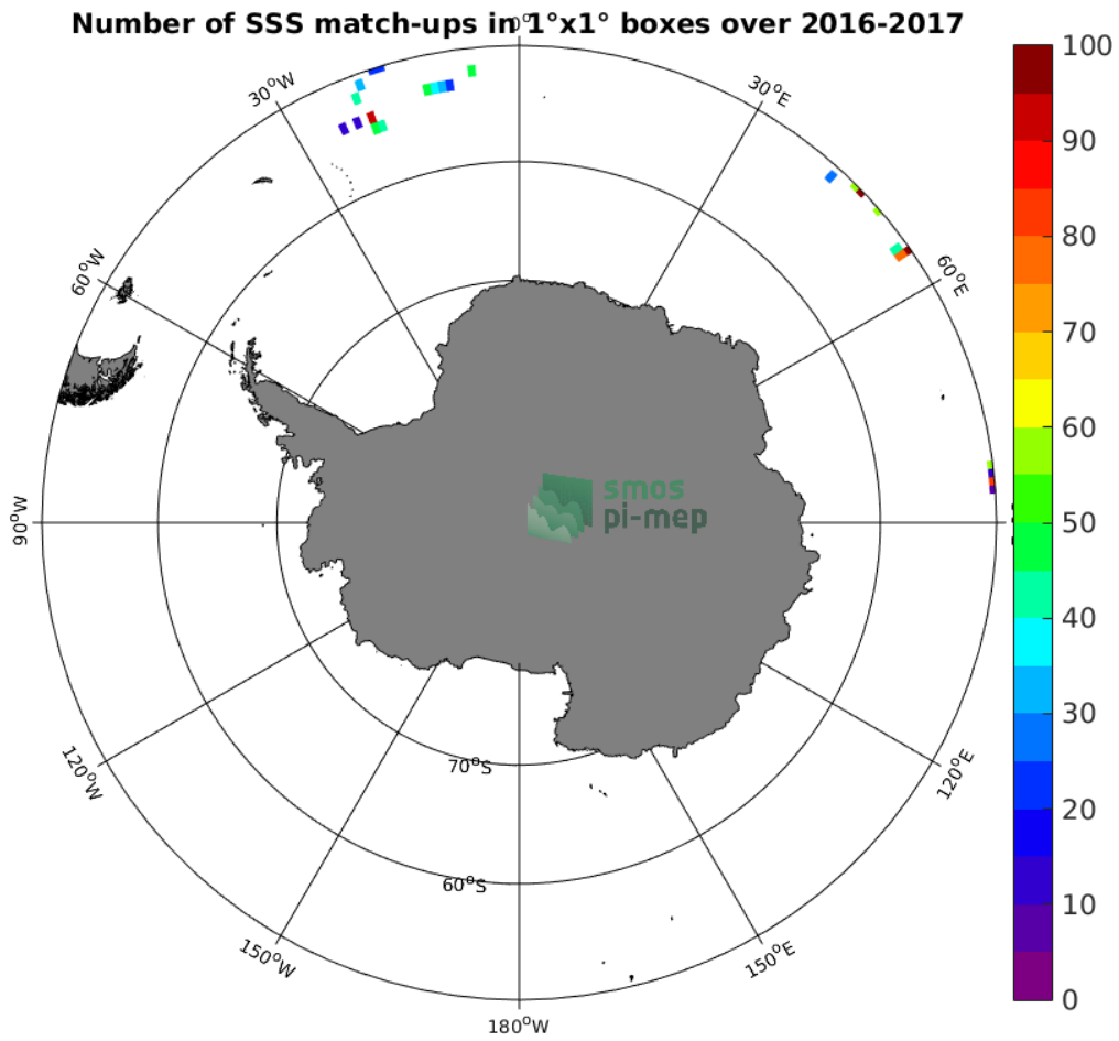
Figure 3: Number of SSS match-ups between Surface drifters SSS and the SMOS-L2-DPGS-v662 SSS product for the Southern Ocean Pi-MEP region over 1°x1° boxes and for the full satellite product period.
