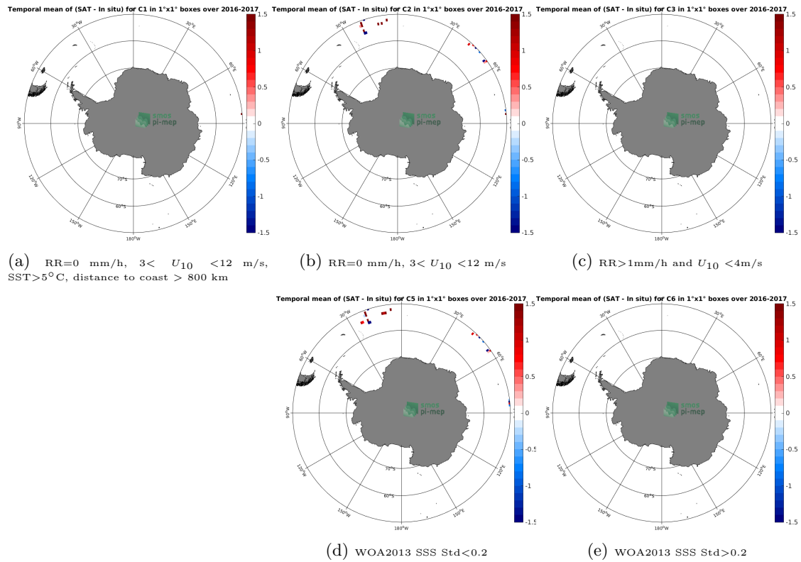
Figure 11: Temporal mean gridded over spatial boxes of size 1^\circ \times 1^\circ of \Delta SSS (SMOS-L2-DPGS-v662 - Surface drifters) for 5 different subdatasets corresponding to:RR=0 mm/h, 3 < U_{10} < 12 m/s, SST >5^\circ C, distance to coast > 800 km (a), RR=0 mm/h, 3 < U_{10} < 12 m/s (b), RR >1 mm/h and U_{10} < 4 m/s (c), WOA2013 SSS Std <0.2 (d), WOA2013 SSS Std >0.2 (e).
