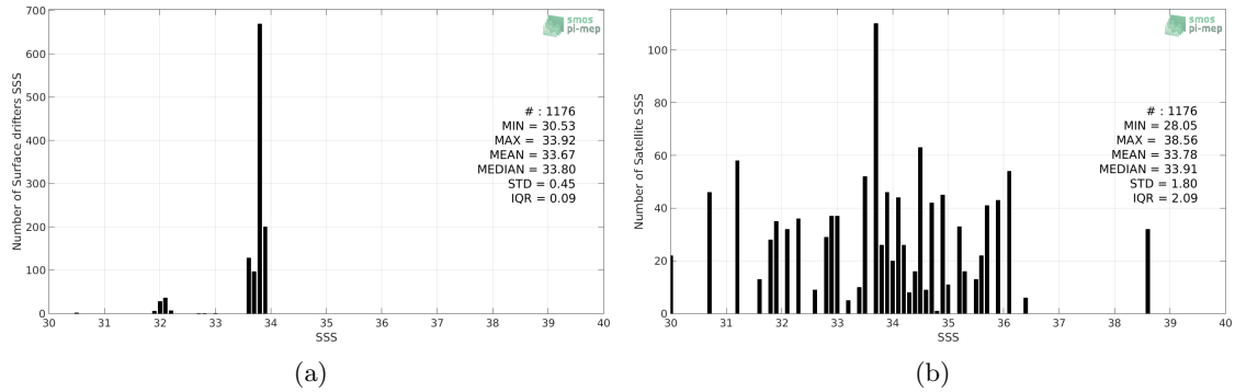
Figure 2: Histograms of SSS from Surface drifters (a) and SMOS-L2-DPGS-v662 (b) considering all match-up pairs per bins of 0.1 over the Southern Ocean Pi-MEP region and for the full satellite product period.
