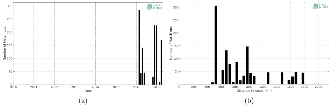
Figure 1: Number of match-ups between Surface drifters and SMOS-L2-DPGS-v662 SSS as a function of time (a) and as function of the distance to coast (b) over the Southern Ocean Pi-MEP region and for the full satellite product period.
