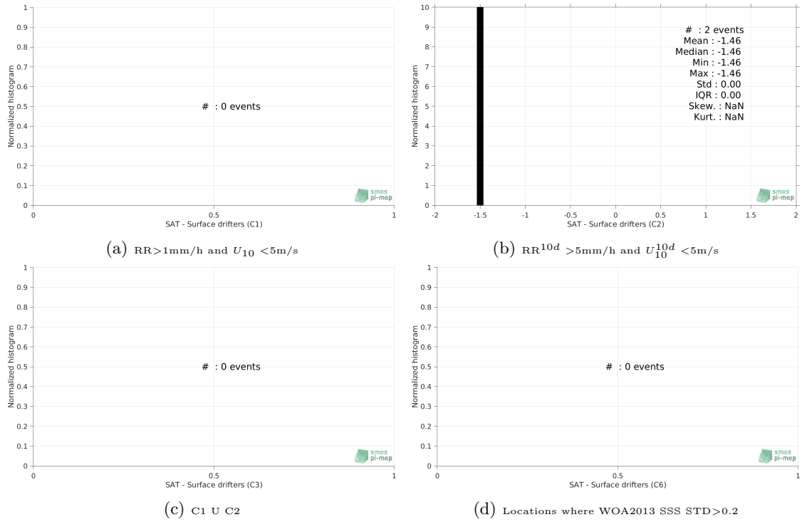
Figure 12: Normalized histogram of \Delta\text{SSS} (SMOS-L2-DPGS-v662 - Surface drifters) for 6 different subdatasets corresponding to: RR > 1\text{mm/h} and U_{10} < 5\text{m/s} (a), RR^{10d} > 5\text{mm/h} and U_{10}^{10d} < 5\text{m/s} (b), C1 \cup C2 (c), Locations where WOA2013 SSS STD > 0.2 (d).
