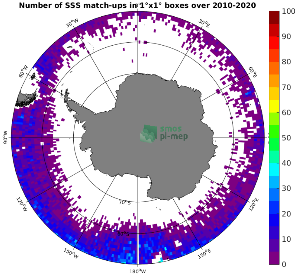
Figure 4: Number of SSS match-ups between Argo SSS and the SMOS SSS L2 v662 (ESA) SSS product for the Southern Ocean Pi-MEP region over 1°x1° boxes and for the full satellite product period.
