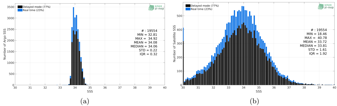
Figure 2: Histograms of SSS from Argo (a) and SMOS L2 v662 (ESA) (b) considering all match-up pairs per bins of 0.1 over the Southern Ocean Pi-MEP region and for the full satellite product period.
