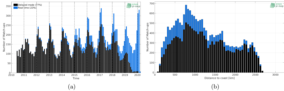
Figure 1: Number of match-ups between Argo and SMOS L2 v662 (ESA) SSS as a function of time (a) and as function of the distance to coast (b) over the Southern Ocean Pi-MEP region and for the full satellite product period.
