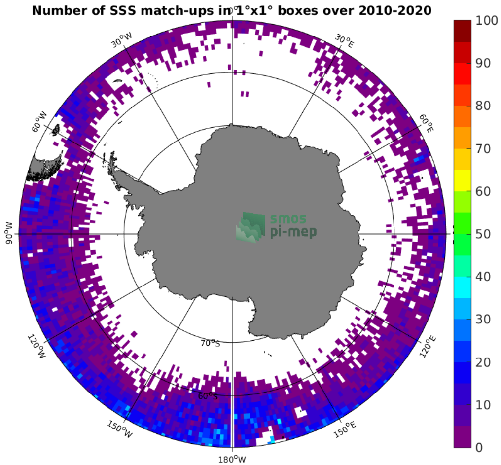
Figure 4: Number of SSS match-ups between Argo SSS and the SMOS L2 v662 (ESA) SSS product for the Southern Ocean Pi-MEP region over 1°x1° boxes and for the full satellite product period.
