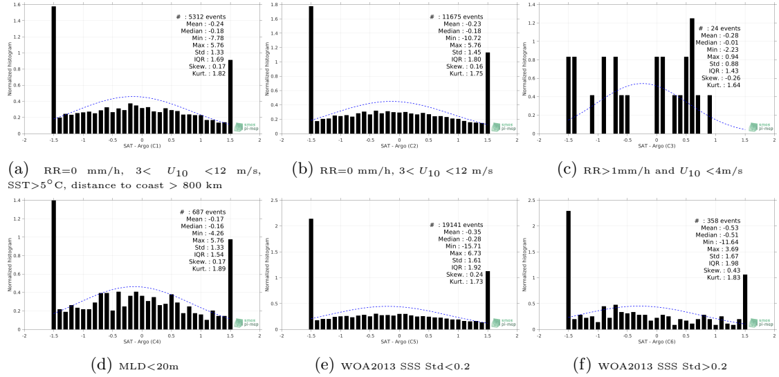
Figure 13: Normalized histogram of \Delta\text{SSS} (SMOS L2 v662 (ESA) - Argo) for 6 different sub-datasets corresponding to: RR=0 mm/h, 3 < U_{10} < 12 m/s, SST>5°C, distance to coast > 800 km (a), RR=0 mm/h, 3 < U_{10} < 12 m/s (b), RR>1mm/h and U_{10} < 4 m/s (c), MLD<20m (d), WOA2013 SSS Std<0.2 (e), WOA2013 SSS Std>0.2 (f).
