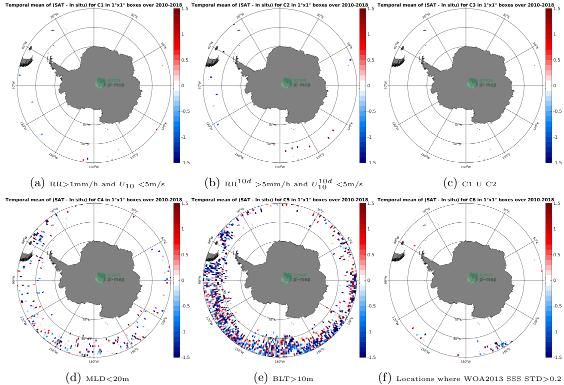
Figure 12: Temporal mean gridded over spatial boxes of size 1^\circ \times 1^\circ of \Delta\text{SSS} (SMOS-L2-DPGS-v662 - Argo) for 6 different subdatasets corresponding to: RR > 1mm/h and U_{10} < 5\text{m/s} (a), RR^{10d} > 5\text{mm/h} and U_{10}^{10d} < 5\text{m/s} (b), C1 U C2 (c), MLD < 20m (d), BLT > 10m (e), Locations where WOA2013 SSS STD > 0.2 (f).
