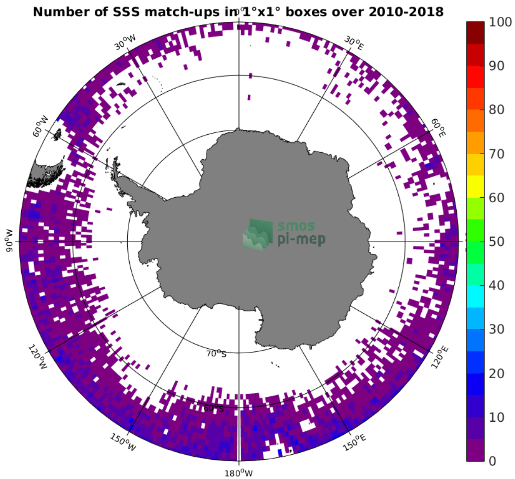
Figure 4: Number of SSS match-ups between Argo SSS and the SMOS-L2-DPGS-v662 SSS product for the Southern Ocean Pi-MEP region over 1^\circ \times 1^\circ boxes and for the full satellite product period.
