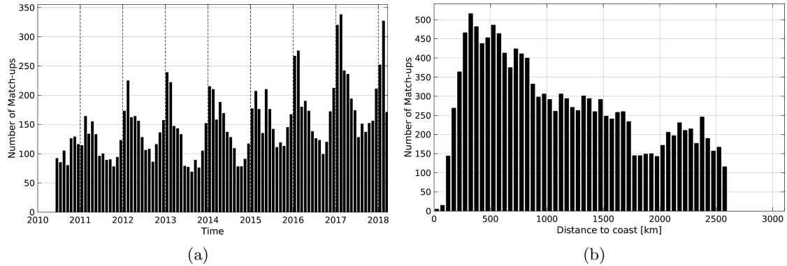
Figure 1: Number of match-ups between Argo and SMOS-L2-DPGS-v662 SSS as a function of time (a) and as function of the distance to coast (b) over the Southern Ocean Pi-MEP region and for the full satellite product period.
