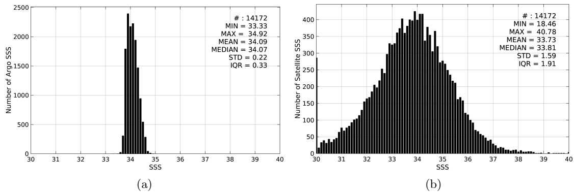
Figure 2: Histograms of SSS from Argo (a) and SMOS-L2-DPGS-v662 (b) considering all match-up pairs per bins of 0.1 over the Southern Ocean Pi-MEP region and for the full satellite product period.
