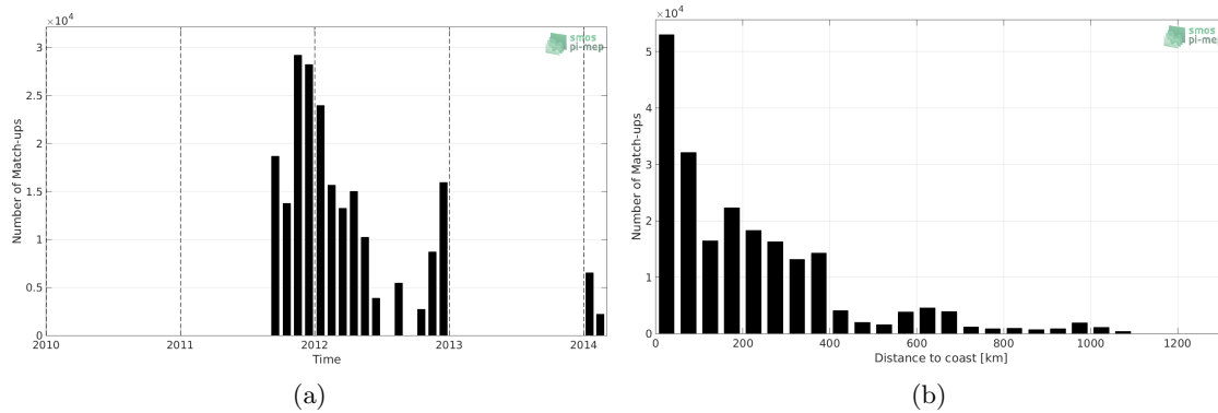
Figure 1: Number of match-ups between TSG (SAMOS) and SMAP SSS L4 OI v1 - 7 Days (IPRC) SSS as a function of time (a) and as function of the distance to coast (b) over the Southern Ocean Pi-MEP region and for the full satellite product period.
