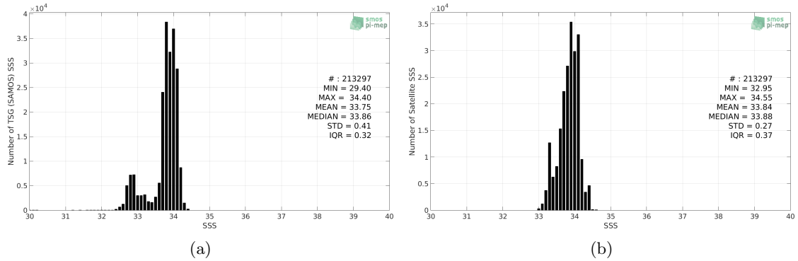
Figure 2: Histograms of SSS from TSG (SAMOS) (a) and SMAP SSS L4 OI v1 - 7 Days (IPRC) (b) considering all match-up pairs per bins of 0.1 over the Southern Ocean Pi-MEP region and for the full satellite product period.
