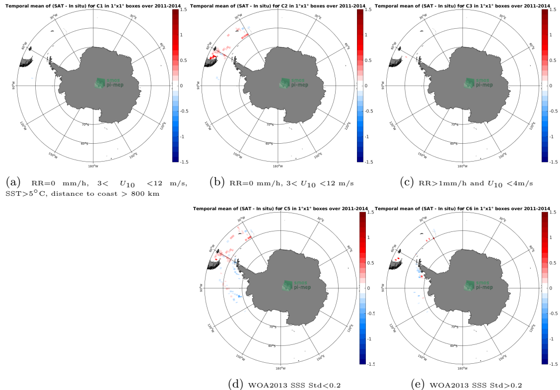
Figure 12: Temporal mean gridded over spatial boxes of size 1^{\circ}\times 1^{\circ} of \Delta\text{SSS} (SMAP SSS L4 OI v1 - 7day (IPRC) - TSG (SAMOS)) for 5 different subdatasets corresponding to:RR=0 mm/h, 3 < U_{10} < 12 m/s, SST >5^{\circ}\text{C} , distance to coast > 800 km (a), RR=0 mm/h, 3 < U_{10} < 12 m/s (b), RR >1 mm/h and U_{10} < 4 m/s (c), WOA2013 SSS Std <0.2 (d), WOA2013 SSS Std >0.2 (e).
