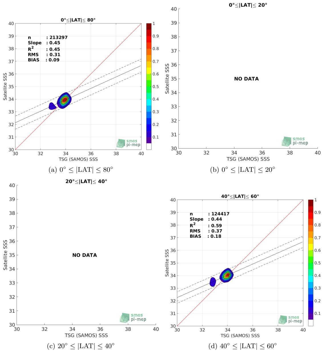
Figure 9: Contour maps of the concentration of SMAP SSS L4 OI v1 - 7day (IPRC) SSS (y-axis) versus TSG (SAMOS) SSS (x-axis) at match-up pairs for different latitude bands. For each plot, the red line shows x=y . The black thin and dashed lines indicate a linear fit through the data cloud and the \pm 95\% confidence levels, respectively. The number match-up pairs n , the slope and R^2 coefficient of the linear fit, the root mean square (RMS) and the mean bias between satellite and in situ data are indicated for each latitude band in each plots.
