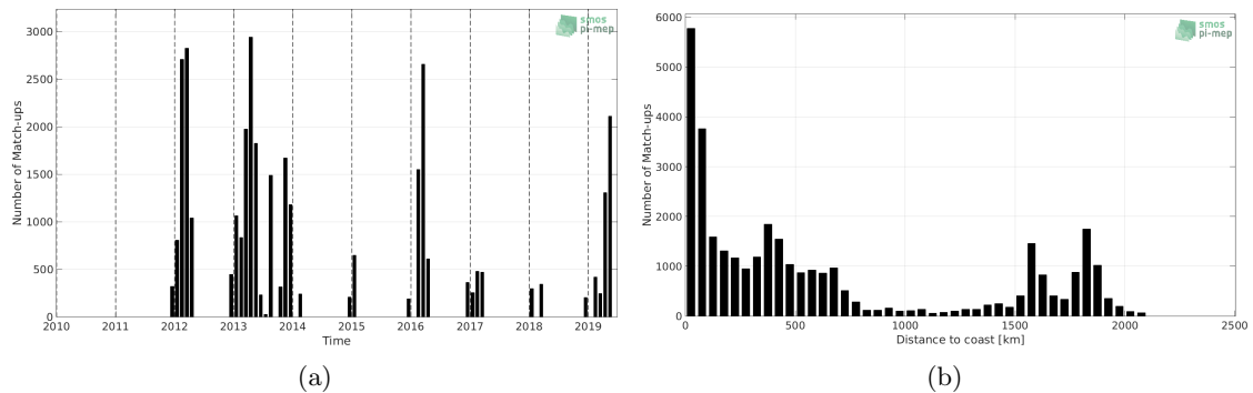
Figure 1: Number of match-ups between TSG (Polarstern) and SMAP SSS L4 OI v1 - 7day (IPRC) SSS as a function of time (a) and as function of the distance to coast (b) over the Southern Ocean Pi-MEP region and for the full satellite product period.
