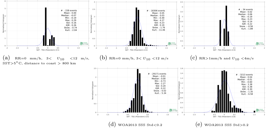
Figure 13: Normalized histogram of \Delta\text{SSS} (SMAP SSS L4 OI v1 - 7day (IPRC) - TSG (Polarstern)) for 5 different subdatasets corresponding to: RR=0 mm/h, 3 < U_{10} < 12 m/s, SST>5°C, distance to coast > 800 km (a), RR=0 mm/h, 3 < U_{10} < 12 m/s (b), RR>1mm/h and U_{10} < 4 m/s (c), WOA2013 SSS Std<0.2 (d), WOA2013 SSS Std>0.2 (e).
