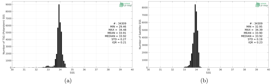
Figure 2: Histograms of SSS from TSG (Polarstern) (a) and SMAP SSS L4 OI v1 - 7day (IPRC) (b) considering all match-up pairs per bins of 0.1 over the Southern Ocean Pi-MEP region and for the full satellite product period.
