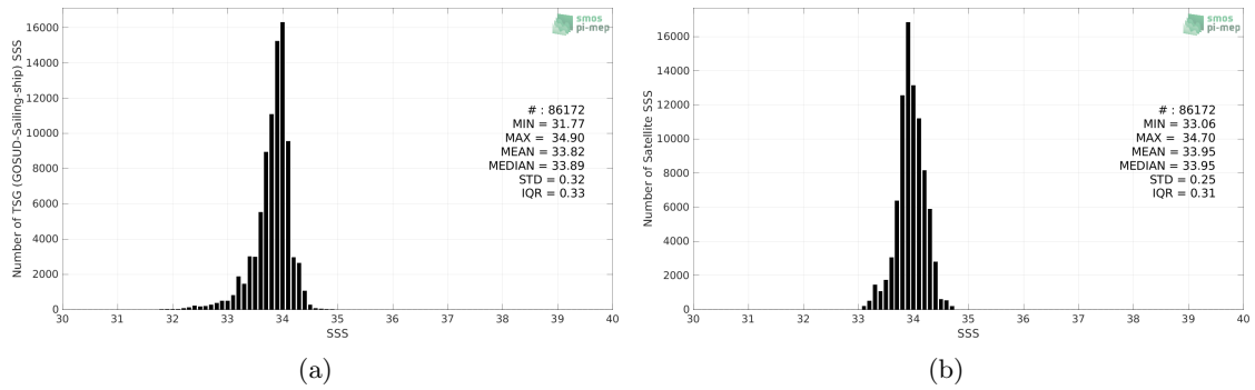
Figure 2: Histograms of SSS from TSG (GOSUD-Sailing-ship) (a) and SMAP SSS L4 OI v1 - 7 Days (IPRC) (b) considering all match-up pairs per bins of 0.1 over the Southern Ocean Pi-MEP region and for the full satellite product period.
