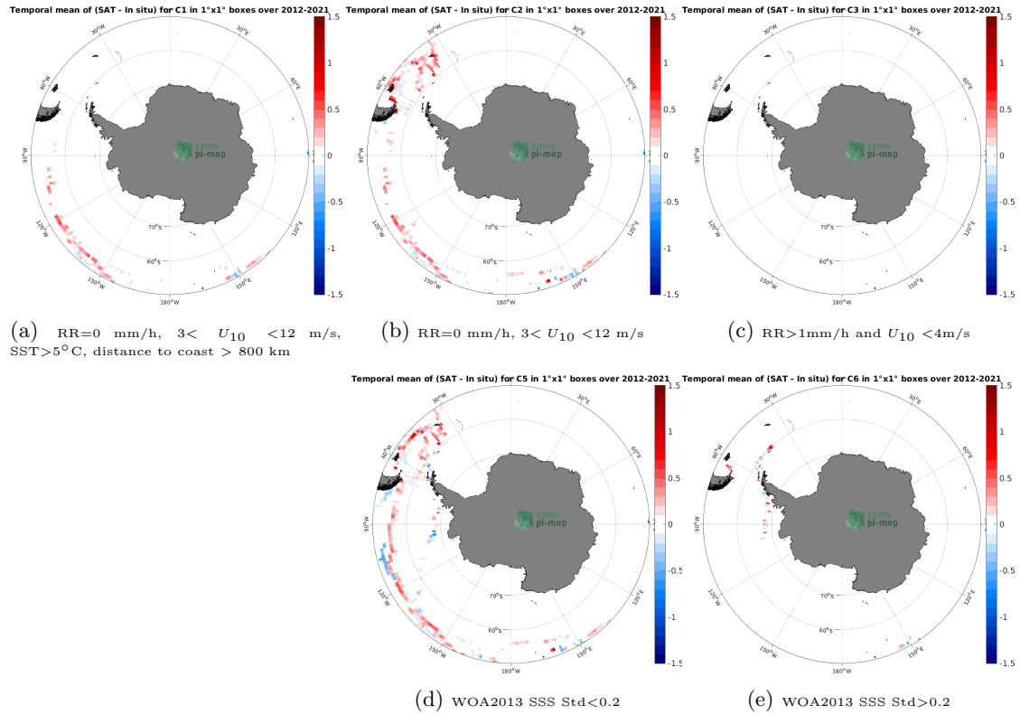
Figure 12: Temporal mean gridded over spatial boxes of size 1^{\circ} \times 1^{\circ} of \Delta SSS (SMAP SSS L4 OI v1 - 7 Days (IPRC) - TSG (GOSUD-Sailing-ship)) for 5 different subdatasets corresponding to: RR=0 mm/h, 3 < U_{10} < 12 m/s, SST >5^{\circ} C, distance to coast > 800 km (a), RR=0 mm/h, 3 < U_{10} < 12 m/s (b), RR >1 mm/h and U_{10} < 4 m/s (c), WOA2013 SSS Std <0.2 (d), WOA2013 SSS Std >0.2 (e).
