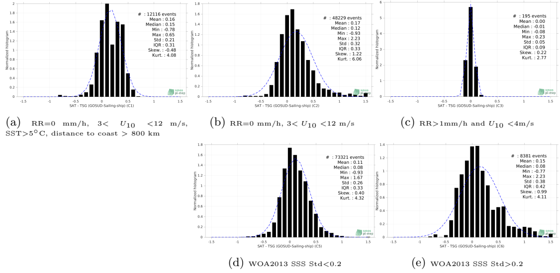
Figure 13: Normalized histogram of \Delta\text{SSS} (SMAP SSS L4 OI v1 - 7 Days (IPRC) - TSG (GOSUD-Sailing-ship)) for 5 different subdatasets corresponding to: RR=0 mm/h, 3 < U_{10} < 12 m/s, SST>5°C, distance to coast > 800 km (a), RR=0 mm/h, 3 < U_{10} < 12 m/s (b), RR>1mm/h and U_{10} < 4 m/s (c), WOA2013 SSS Std<0.2 (d), WOA2013 SSS Std>0.2 (e).
