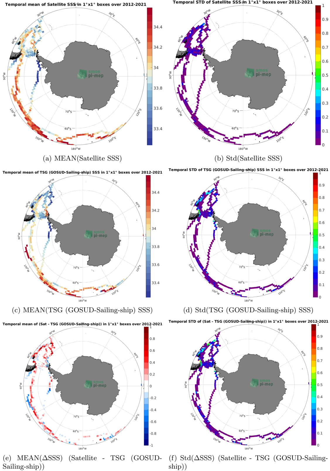
Figure 6: Temporal mean (left) and Std (right) of SSS from SMAP SSS L4 OI v1 - 7 Days (IPRC) (top), TSG (GOSUD-Sailing-ship) (middle), and of \Delta SSS (Satellite - TSG (GOSUD-Sailing-ship)). Only match-up pairs are used to generate these maps.
