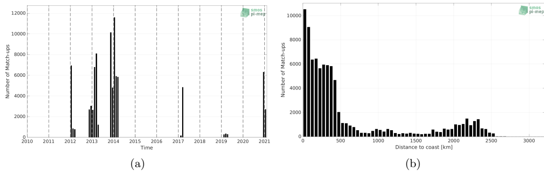
Figure 1: Number of match-ups between TSG (GOSUD-Sailing-ship) and SMAP SSS L4 OI v1 - 7 Days (IPRC) SSS as a function of time (a) and as function of the distance to coast (b) over the Southern Ocean Pi-MEP region and for the full satellite product period.
