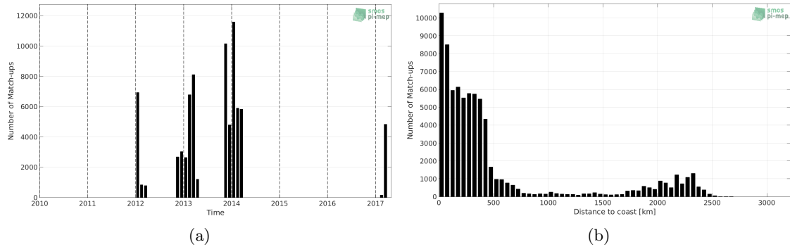
Figure 1: Number of match-ups between TSG (GOSUD-Sailing-ship) and SMAP SSS L4 OI v1 - 7day (IPRC) SSS as a function of time (a) and as function of the distance to coast (b) over the Southern Ocean Pi-MEP region and for the full satellite product period.
