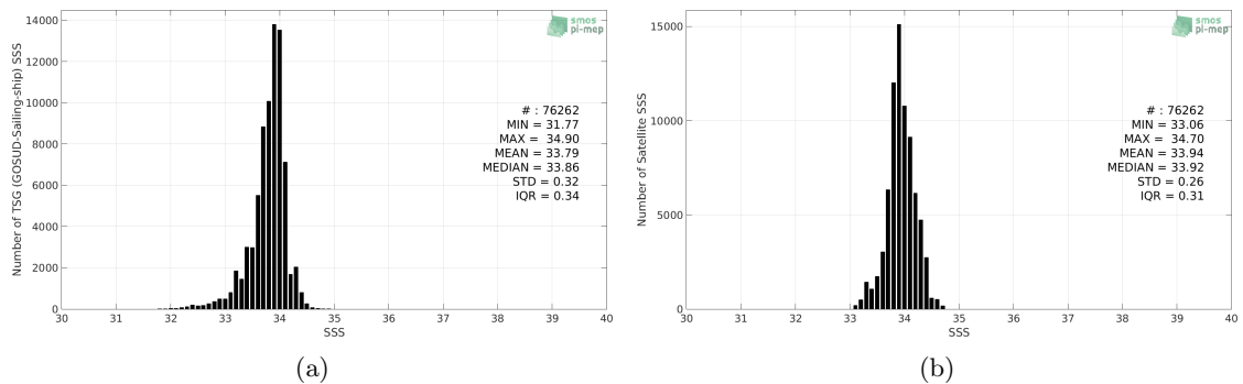
Figure 2: Histograms of SSS from TSG (GOSUD-Sailing-ship) (a) and SMAP SSS L4 OI v1 - 7day (IPRC) (b) considering all match-up pairs per bins of 0.1 over the Southern Ocean Pi-MEP region and for the full satellite product period.
