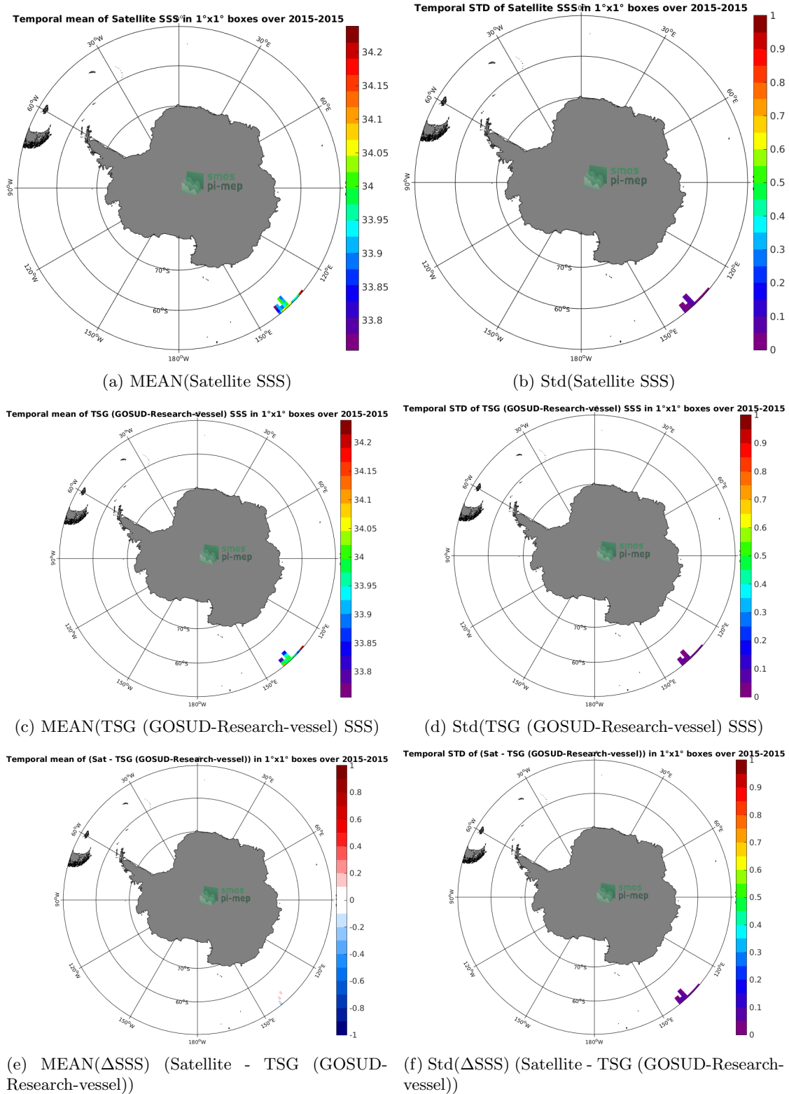
Figure 6: Temporal mean (left) and Std (right) of SSS from SMAP SSS L4 OI v1 - 7 Days (IPRC) (top), TSG (GOSUD-Research-vessel) (middle), and of \Delta SSS (Satellite - TSG (GOSUD-Research-vessel)). Only match-up pairs are used to generate these maps.
