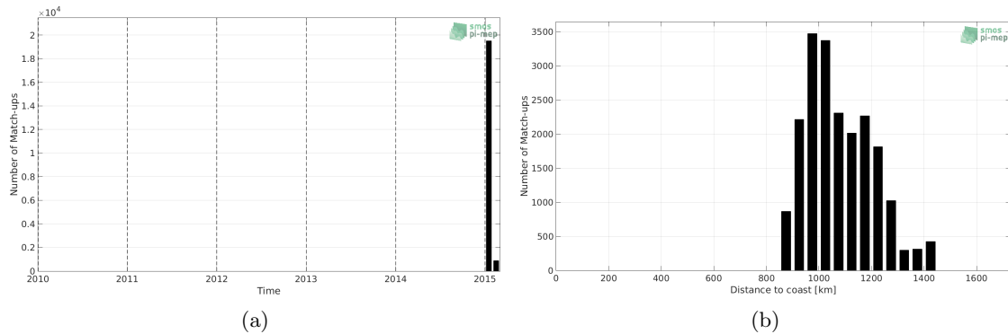
Figure 1: Number of match-ups between TSG (GOSUD-Research-vessel) and SMAP SSS L4 OI v1 - 7 Days (IPRC) SSS as a function of time (a) and as function of the distance to coast (b) over the Southern Ocean Pi-MEP region and for the full satellite product period.
