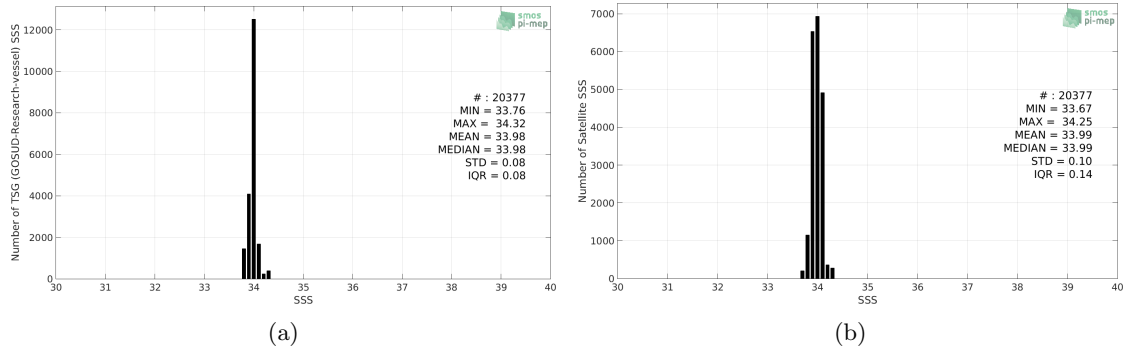
Figure 2: Histograms of SSS from TSG (GOSUD-Research-vessel) (a) and SMAP SSS L4 OI v1 - 7 Days (IPRC) (b) considering all match-up pairs per bins of 0.1 over the Southern Ocean Pi-MEP region and for the full satellite product period.
