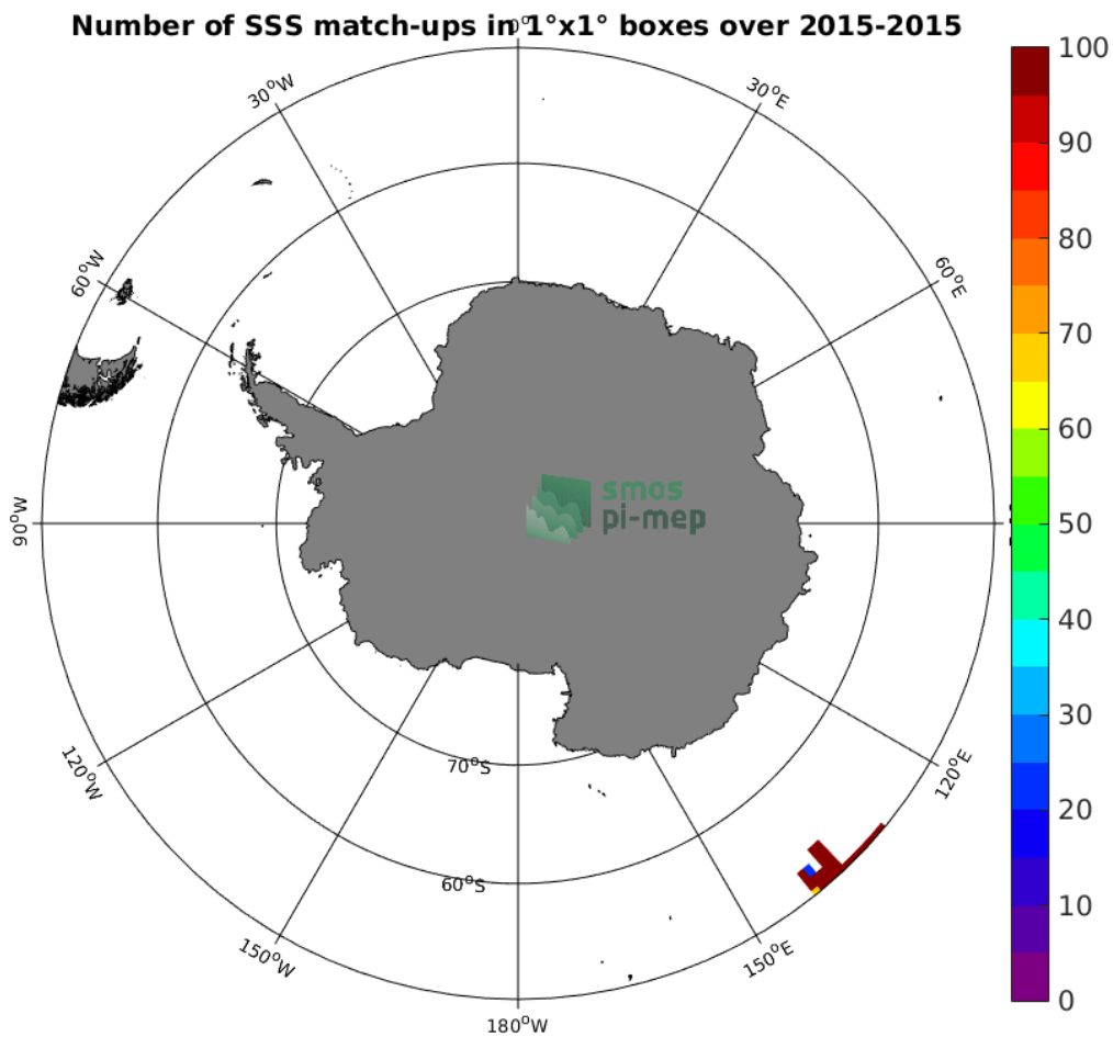
Figure 4: Number of SSS match-ups between TSG (GOSUD-Research-vessel) SSS and the SMAP SSS L4 OI v1 - 7 Days (IPRC) SSS product for the Southern Ocean Pi-MEP region over 1^\circ \times 1^\circ boxes and for the full satellite product period.
