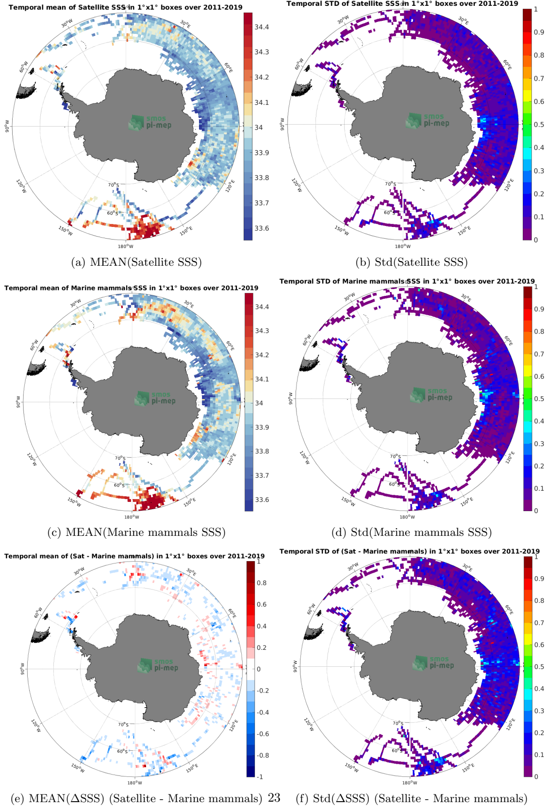
Figure 6: Temporal mean (left) and Std (right) of SSS from SMAP SSS L4 OI v1 - 7 Days (IPRC) (top), Marine mammals (middle), and of \Delta SSS (Satellite - Marine mammals). Only match-up pairs are used to generate these maps.
