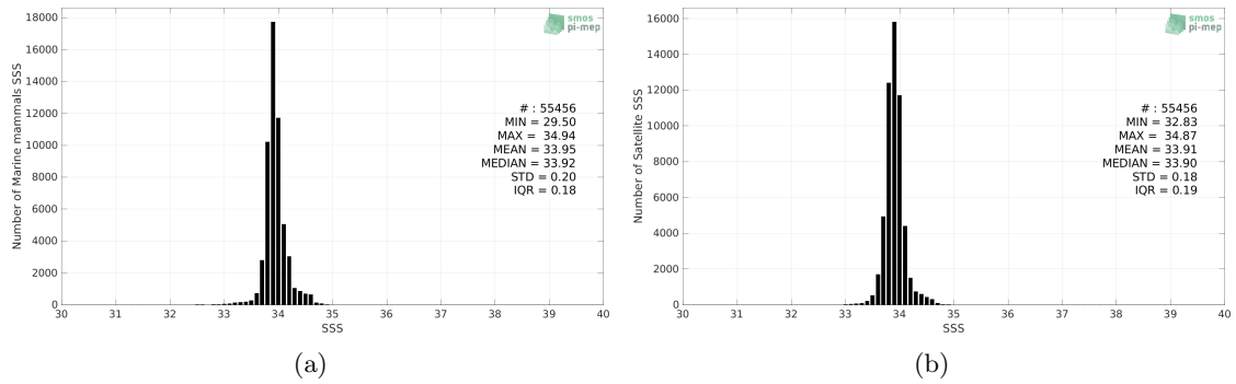
Figure 2: Histograms of SSS from Marine mammals (a) and SMAP SSS L4 OI v1 - 7 Days (IPRC) (b) considering all match-up pairs per bins of 0.1 over the Southern Ocean Pi-MEP region and for the full satellite product period.
