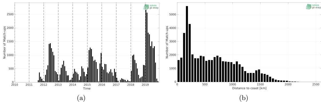
Figure 1: Number of match-ups between Marine mammals and SMAP SSS L4 OI v1 - 7 Days (IPRC) SSS as a function of time (a) and as function of the distance to coast (b) over the Southern Ocean Pi-MEP region and for the full satellite product period.
