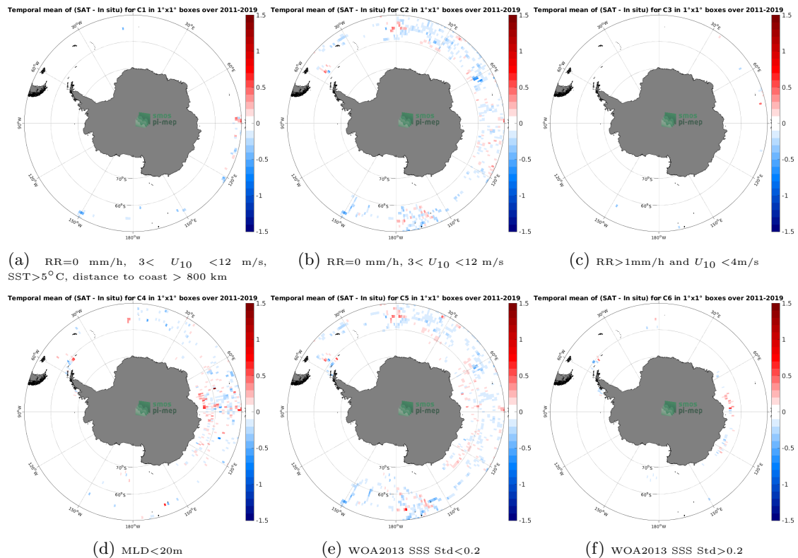
Figure 12: Temporal mean gridded over spatial boxes of size 1^{\circ}\times 1^{\circ} of \Delta\text{SSS} (SMAP SSS L4 OI v1 - 7 Days (IPRC) - Marine mammals) for 6 different subdatasets corresponding to:RR=0 mm/h, 3 < U_{10} < 12 m/s, SST >5^{\circ}\text{C} , distance to coast > 800 km (a), RR=0 mm/h, 3 < U_{10} < 12 m/s (b), RR >1 mm/h and U_{10} < 4 m/s (c),MLD <20 m (d),WOA2013 SSS Std <0.2 (e),WOA2013 SSS Std >0.2 (f).
