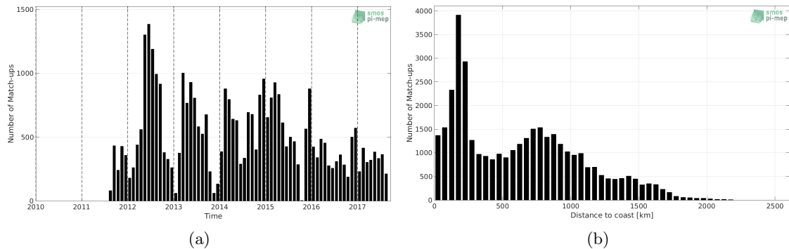
Figure 1: Number of match-ups between Sea mammals and SMAP SSS L4 OI v1 - 7day (IPRC) SSS as a function of time (a) and as function of the distance to coast (b) over the Southern Ocean Pi-MEP region and for the full satellite product period.
