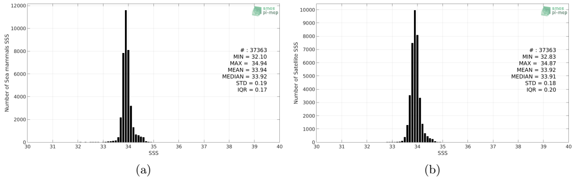
Figure 2: Histograms of SSS from Sea mammals (a) and SMAP SSS L4 OI v1 - 7day (IPRC) (b) considering all match-up pairs per bins of 0.1 over the Southern Ocean Pi-MEP region and for the full satellite product period.
