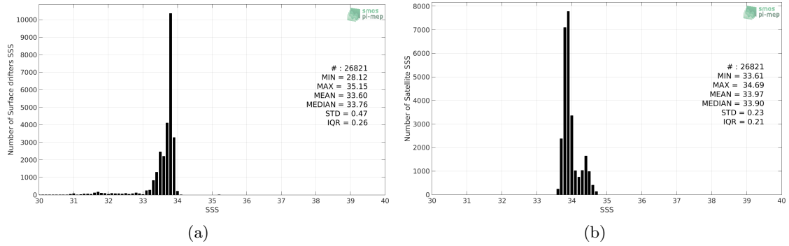
Figure 2: Histograms of SSS from Surface drifters (a) and SMAP SSS L4 OI v1 - 7 Days (IPRC) (b) considering all match-up pairs per bins of 0.1 over the Southern Ocean Pi-MEP region and for the full satellite product period.
