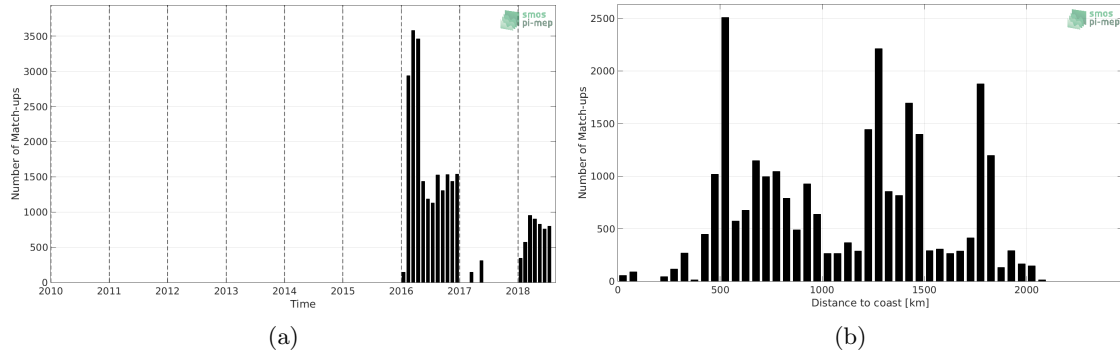
Figure 1: Number of match-ups between Surface drifters and SMAP SSS L4 OI v1 - 7 Days (IPRC) SSS as a function of time (a) and as function of the distance to coast (b) over the Southern Ocean Pi-MEP region and for the full satellite product period.
