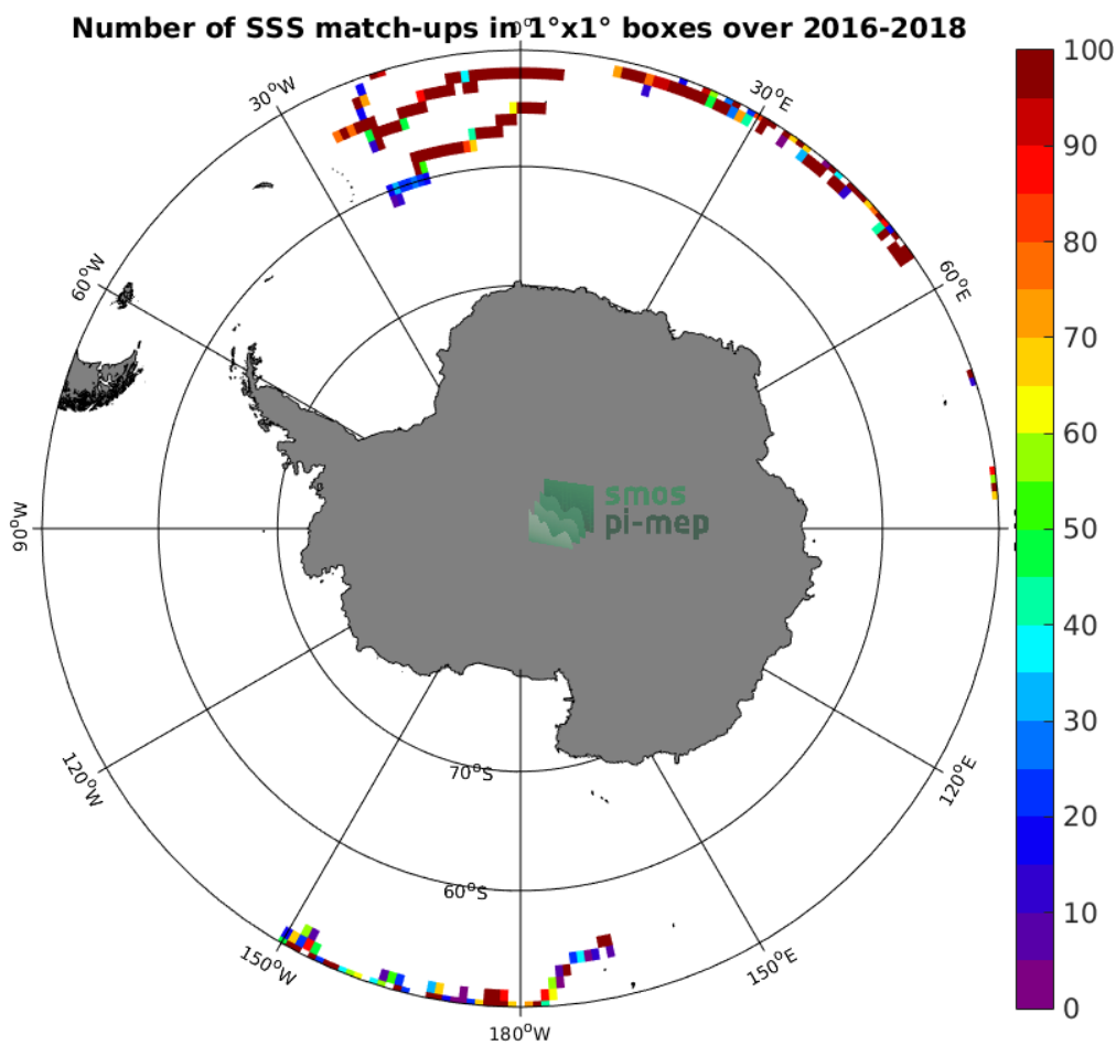
Figure 3: Number of SSS match-ups between Surface drifters SSS and the SMAP SSS L4 OI v1 - 7 Days (IPRC) SSS product for the Southern Ocean Pi-MEP region over 1^\circ \times 1^\circ boxes and for the full satellite product period.
