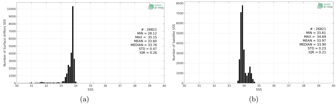
Figure 2: Histograms of SSS from Surface drifters (a) and SMAP SSS L4 OI v1 - 7day (IPRC) (b) considering all match-up pairs per bins of 0.1 over the Southern Ocean Pi-MEP region and for the full satellite product period.
