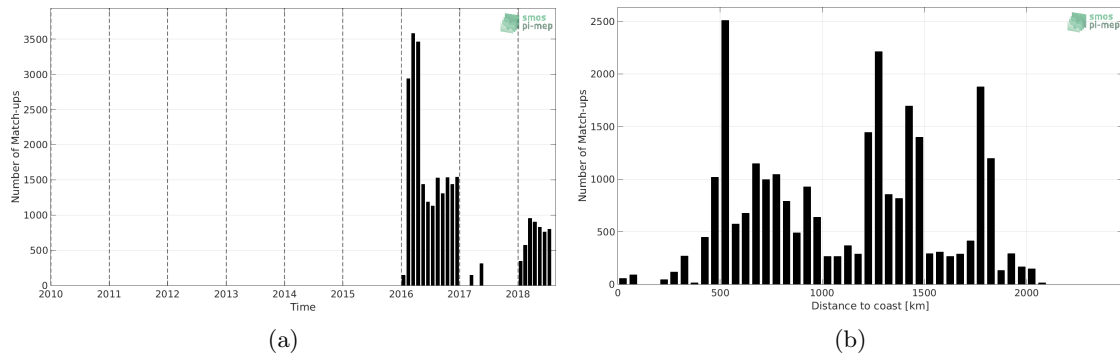
Figure 1: Number of match-ups between Surface drifters and SMAP SSS L4 OI v1 - 7day (IPRC) SSS as a function of time (a) and as function of the distance to coast (b) over the Southern Ocean Pi-MEP region and for the full satellite product period.
