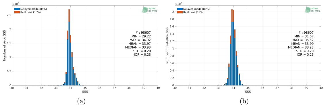
Figure 2: Histograms of SSS from Argo (a) and SMAP SSS L4 OI v1 - 7 Days (IPRC) (b) considering all match-up pairs per bins of 0.1 over the Southern Ocean Pi-MEP region and for the full satellite product period.
