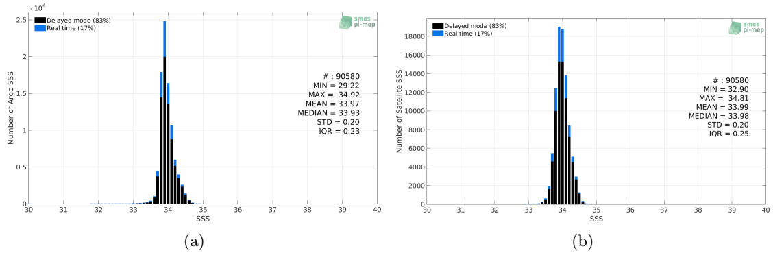
Figure 2: Histograms of SSS from Argo (a) and SMAP SSS L4 OI v1 - 7day (IPRC) (b) considering all match-up pairs per bins of 0.1 over the Southern Ocean Pi-MEP region and for the full satellite product period.
