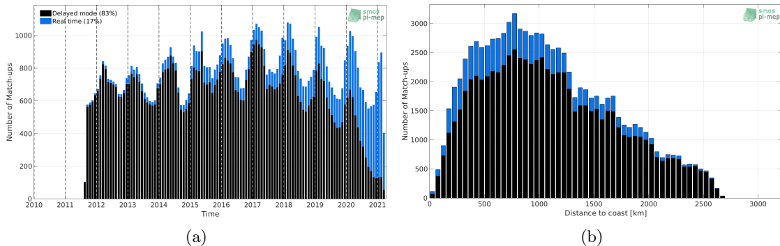
Figure 1: Number of match-ups between Argo and SMAP SSS L4 OI v1 - 7day (IPRC) SSS as a function of time (a) and as function of the distance to coast (b) over the Southern Ocean Pi-MEP region and for the full satellite product period.
