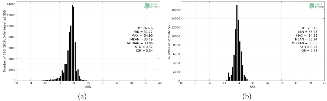
Figure 2: Histograms of SSS from TSG (GOSUD-Sailing-ship) (a) and SMAP SSS L4 OI v1 - Monthly (IPRC) (b) considering all match-up pairs per bins of 0.1 over the Southern Ocean Pi-MEP region and for the full satellite product period.
