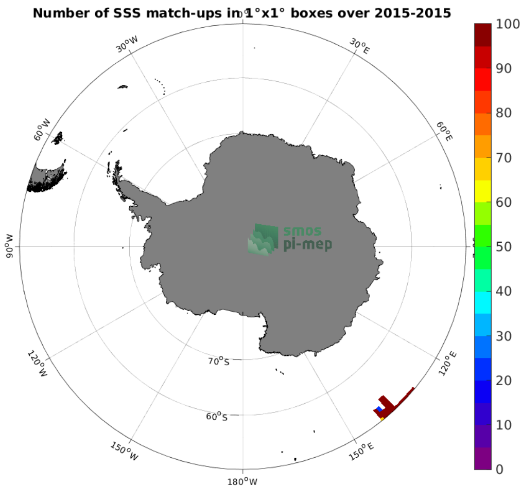
Figure 4: Number of SSS match-ups between TSG (GOSUD-Research-vessel) SSS and the SMAP SSS L4 OI v1 - Monthly (IPRC) SSS product for the Southern Ocean Pi-MEP region over 1^{\circ} \times 1^{\circ} boxes and for the full satellite product period.
