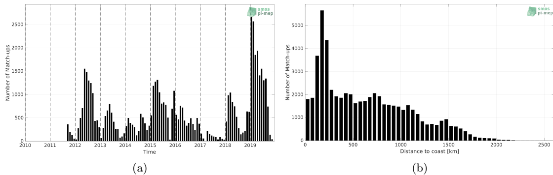
Figure 1: Number of match-ups between Marine mammals and SMAP SSS L4 OI v1 - Monthly (IPRC) SSS as a function of time (a) and as function of the distance to coast (b) over the Southern Ocean Pi-MEP region and for the full satellite product period.
