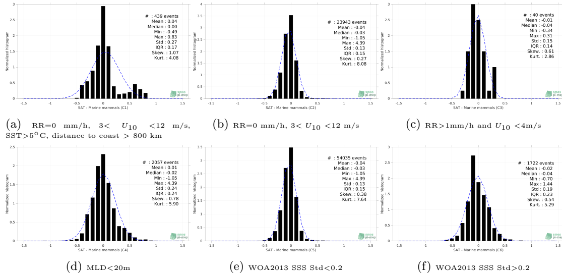
Figure 13: Normalized histogram of \Delta SSS (SMAP SSS L4 OI v1 - Monthly (IPRC) - Marine mammals) for 6 different subdatasets corresponding to: RR=0 mm/h, 3 < U_{10} < 12 m/s, SST > 5°C, distance to coast > 800 km (a), RR=0 mm/h, 3 < U_{10} < 12 m/s (b), RR > 1mm/h and U_{10} < 4 m/s (c), MLD < 20m (d), WOA2013 SSS Std < 0.2 (e), WOA2013 SSS Std > 0.2 (f).
