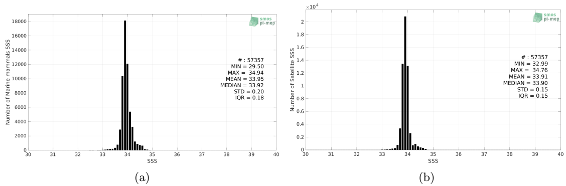
Figure 2: Histograms of SSS from Marine mammals (a) and SMAP SSS L4 OI v1 - Monthly (IPRC) (b) considering all match-up pairs per bins of 0.1 over the Southern Ocean Pi-MEP region and for the full satellite product period.
