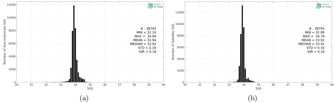
Figure 2: Histograms of SSS from Marine mammals (a) and SMAP SSS L4 OI v1 - Monthly (IPRC) (b) considering all match-up pairs per bins of 0.1 over the Southern Ocean Pi-MEP region and for the full satellite product period.
