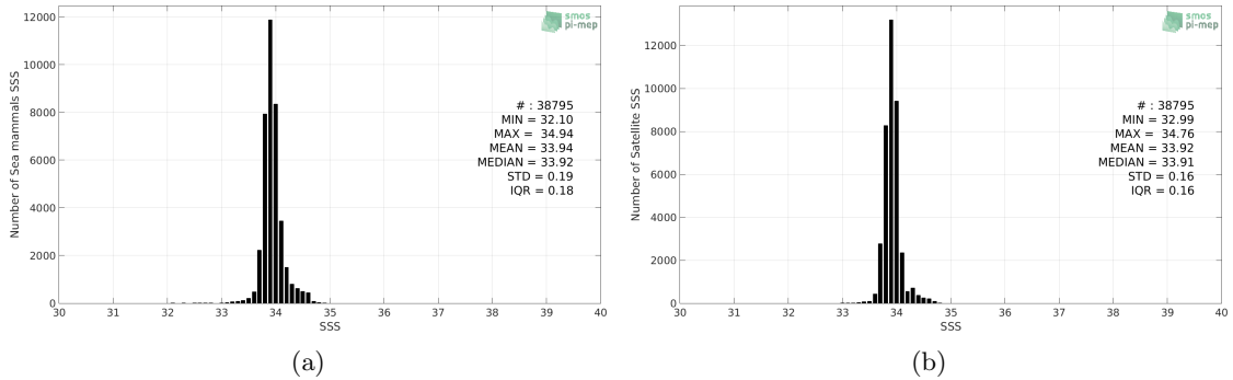
Figure 2: Histograms of SSS from Sea mammals (a) and SMAP SSS L4 OI v1 - Monthly (IPRC) (b) considering all match-up pairs per bins of 0.1 over the Southern Ocean Pi-MEP region and for the full satellite product period.
