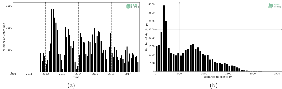
Figure 1: Number of match-ups between Sea mammals and SMAP SSS L4 OI v1 - Monthly (IPRC) SSS as a function of time (a) and as function of the distance to coast (b) over the Southern Ocean Pi-MEP region and for the full satellite product period.
