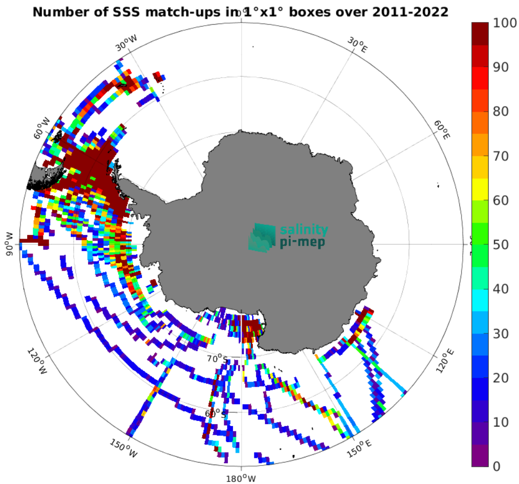
Figure 5: Number of SSS match-ups between TSG (SAMOS) SSS and the SMAP SSS L4 OI v3 - Monthly (ESR) SSS product for the Southern Ocean Pi-MEP region over 1^\circ \times 1^\circ boxes and for the full satellite product period.
