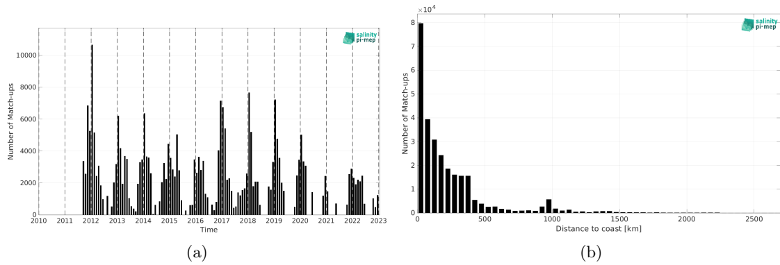
Figure 2: Number of match-ups between TSG (SAMOS) and SMAP SSS L4 OI v3 - Monthly (ESR) SSS as a function of time (a) and as function of the distance to coast (b) over the Southern Ocean Pi-MEP region and for the full satellite product period.
