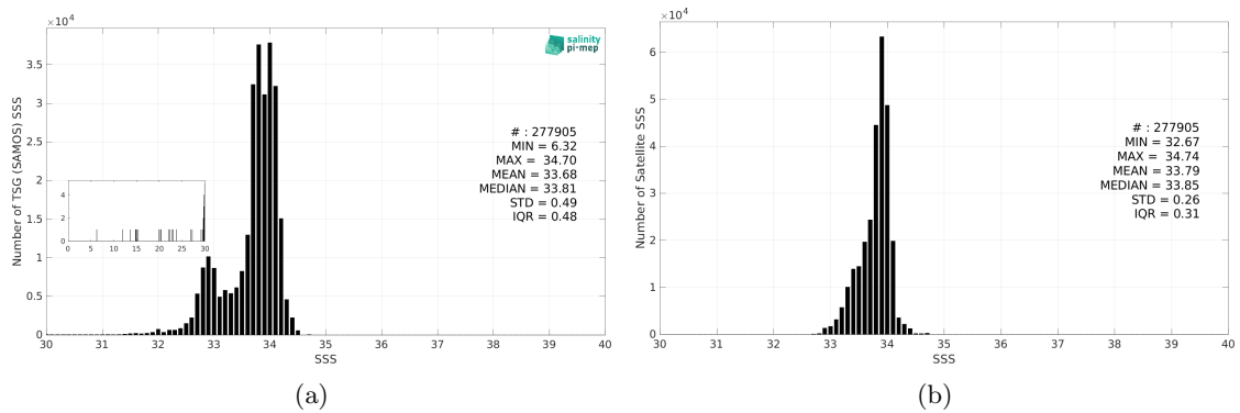
Figure 3: Histograms of SSS from TSG (SAMOS) (a) and SMAP SSS L4 OI v3 - Monthly (ESR) (b) considering all match-up pairs per bins of 0.1 over the Southern Ocean Pi-MEP region and for the full satellite product period.
