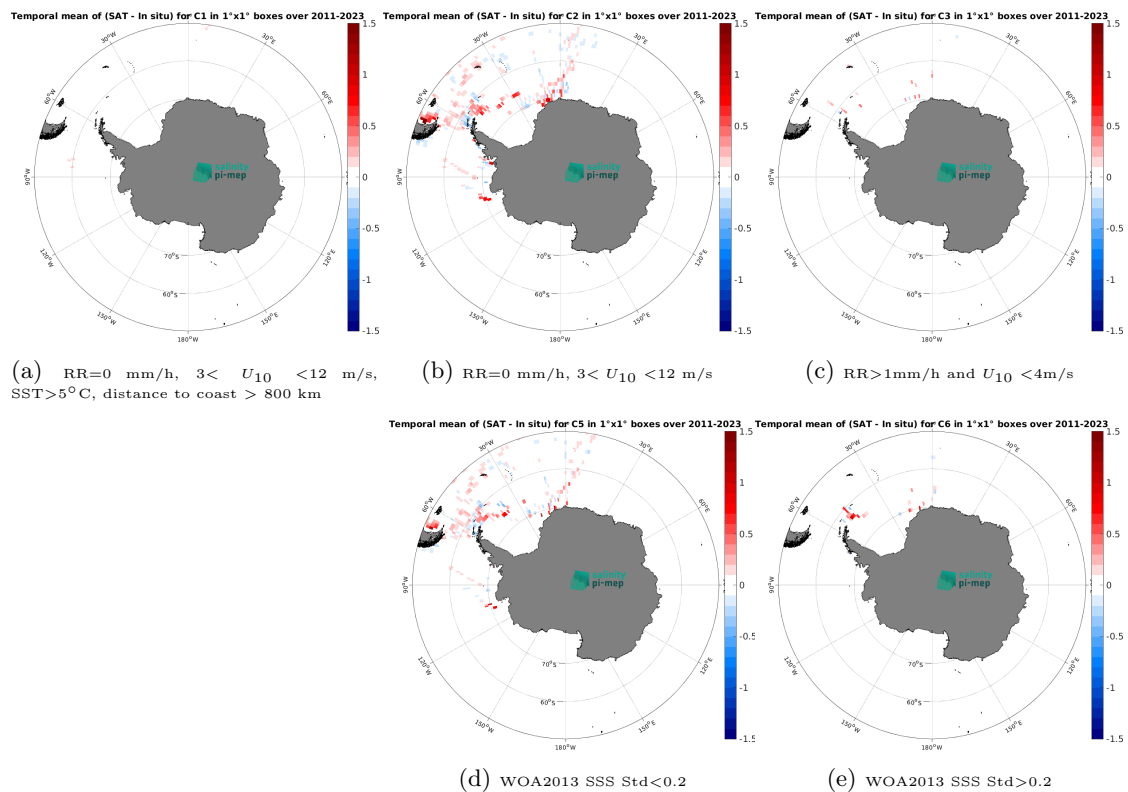
Figure 14: Temporal mean gridded over spatial boxes of size 1^\circ \times 1^\circ of \Delta SSS (SMAP SSS L4 OI v3 - Monthly (ESR) - TSG (Polarstern)) for 5 different subdatasets corresponding to:RR=0 mm/h, 3 < U_{10} < 12 m/s, SST > 5^\circ\text{C} , distance to coast > 800 km (a), RR=0 mm/h, 3 < U_{10} < 12 m/s (b), RR > 1 mm/h and U_{10} < 4 m/s (c), WOA2013 SSS Std < 0.2 (d), WOA2013 SSS Std > 0.2 (e).
