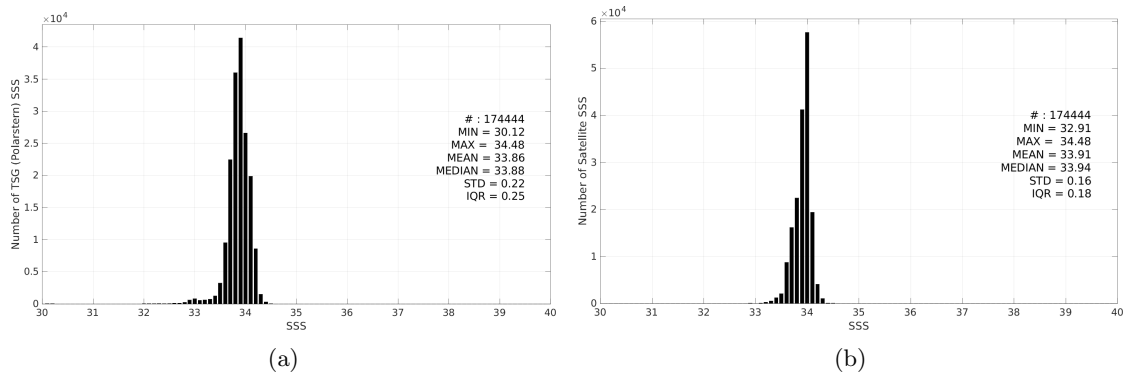
Figure 3: Histograms of SSS from TSG (Polarstern) (a) and SMAP SSS L4 OI v3 - Monthly (ESR) (b) considering all match-up pairs per bins of 0.1 over the Southern Ocean Pi-MEP region and for the full satellite product period.
