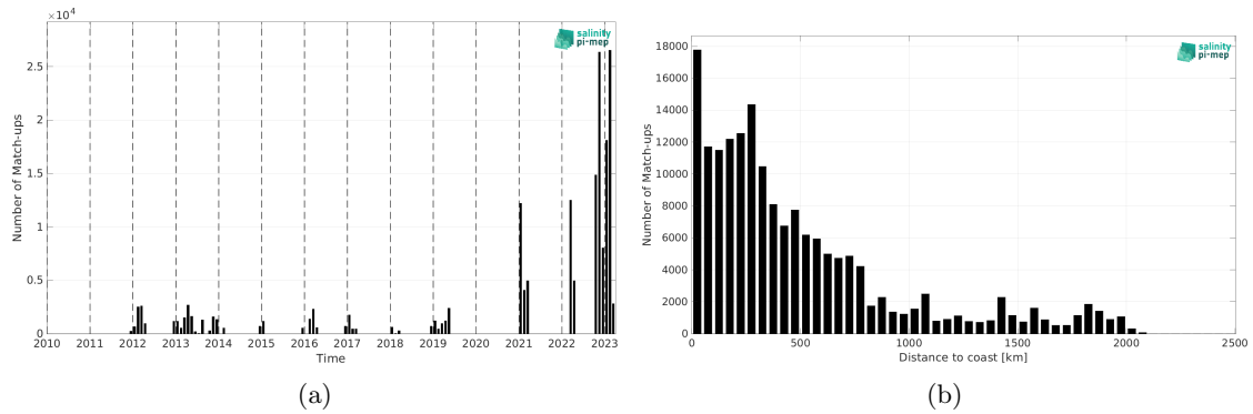
Figure 2: Number of match-ups between TSG (Polarstern) and SMAP SSS L4 OI v3 - Monthly (ESR) SSS as a function of time (a) and as function of the distance to coast (b) over the Southern Ocean Pi-MEP region and for the full satellite product period.
