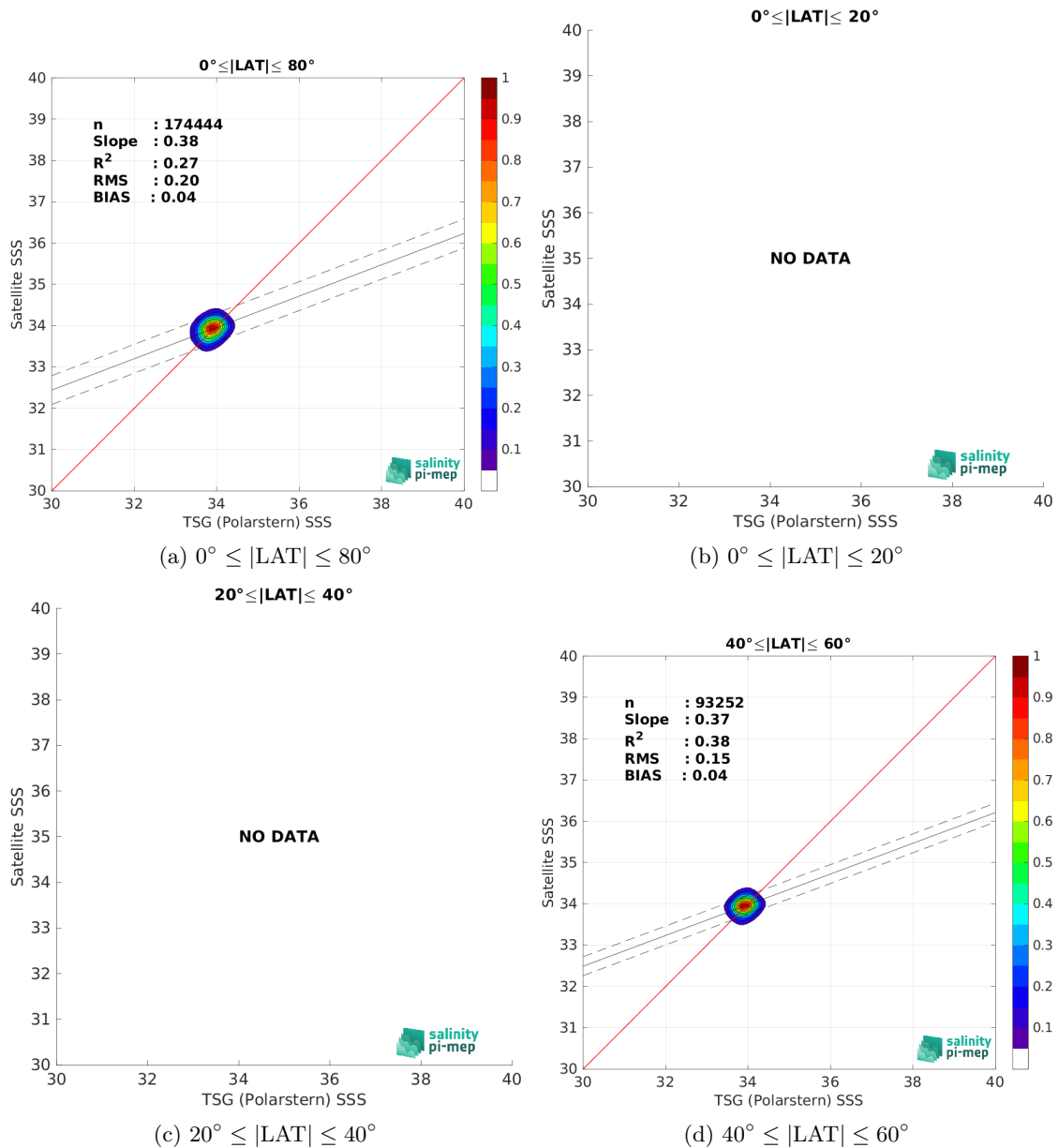
Figure 10: Contour maps of the concentration of SMAP SSS L4 OI v3 - Monthly (ESR) SSS (y-axis) versus TSG (Polarstern) SSS (x-axis) at match-up pairs for different latitude bands. For each plot, the red line shows x=y . The black thin and dashed lines indicate a linear fit through the data cloud and the \pm 95\% confidence levels, respectively. The number match-up pairs n , the slope and R^2 coefficient of the linear fit, the root mean square (RMS) and the mean bias between satellite and in situ data are indicated for each latitude band in each plots.
