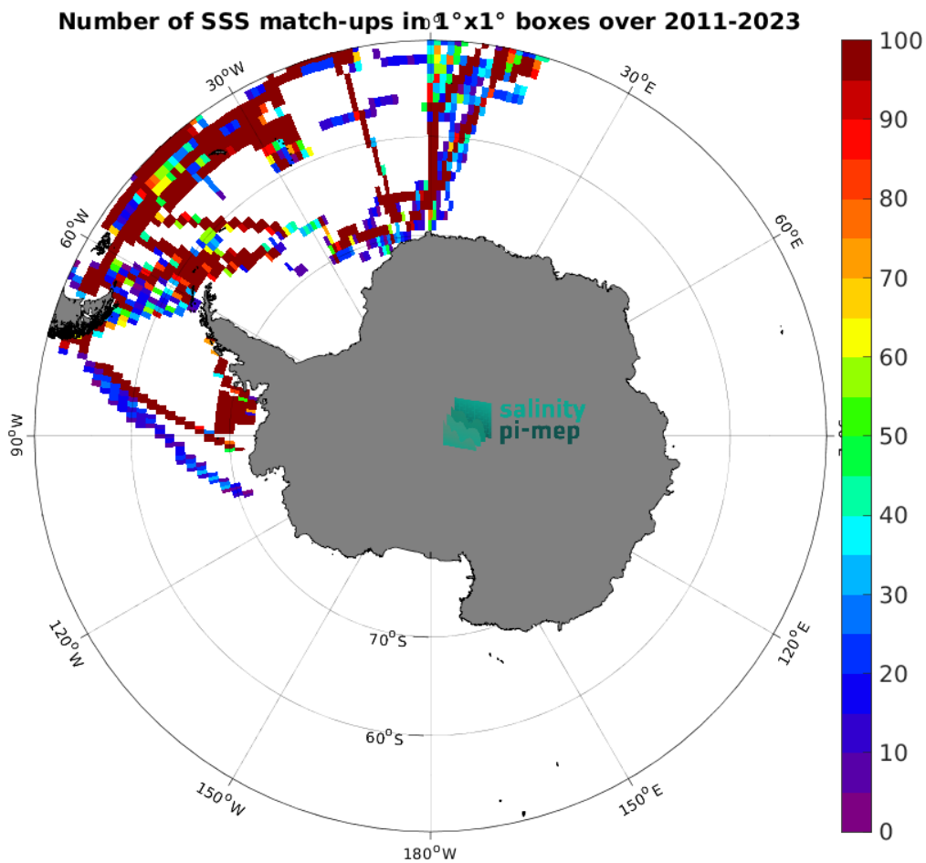
Figure 5: Number of SSS match-ups between TSG (Polarstern) SSS and the SMAP SSS L4 OI v3 - Monthly (ESR) SSS product for the Southern Ocean Pi-MEP region over 1^\circ \times 1^\circ boxes and for the full satellite product period.
