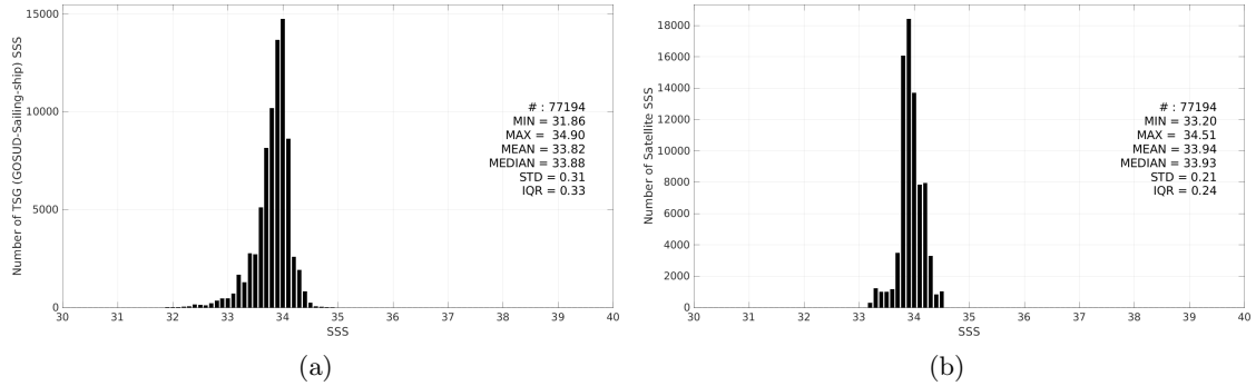
Figure 3: Histograms of SSS from TSG (GOSUD-Sailing-ship) (a) and SMAP SSS L4 OI v3 - Monthly (ESR) (b) considering all match-up pairs per bins of 0.1 over the Southern Ocean Pi-MEP region and for the full satellite product period.
