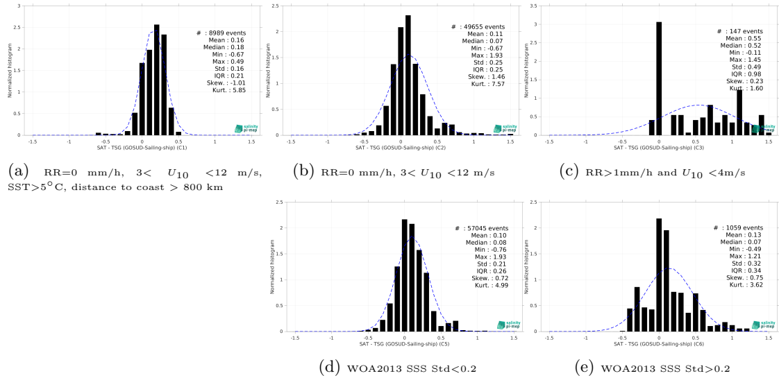
Figure 15: Normalized histogram of \Delta\text{SSS} (SMAP SSS L4 OI v3 - Monthly (ESR) - TSG (GOSUD-Sailing-ship)) for 5 different subdatasets corresponding to: RR=0 mm/h, 3 < U_{10} < 12 m/s, SST >5^{\circ}\text{C} , distance to coast > 800 km (a), RR=0 mm/h, 3 < U_{10} < 12 m/s (b), RR >1 mm/h and U_{10} < 4 m/s (c), WOA2013 SSS Std <0.2 (d), WOA2013 SSS Std >0.2 (e).
