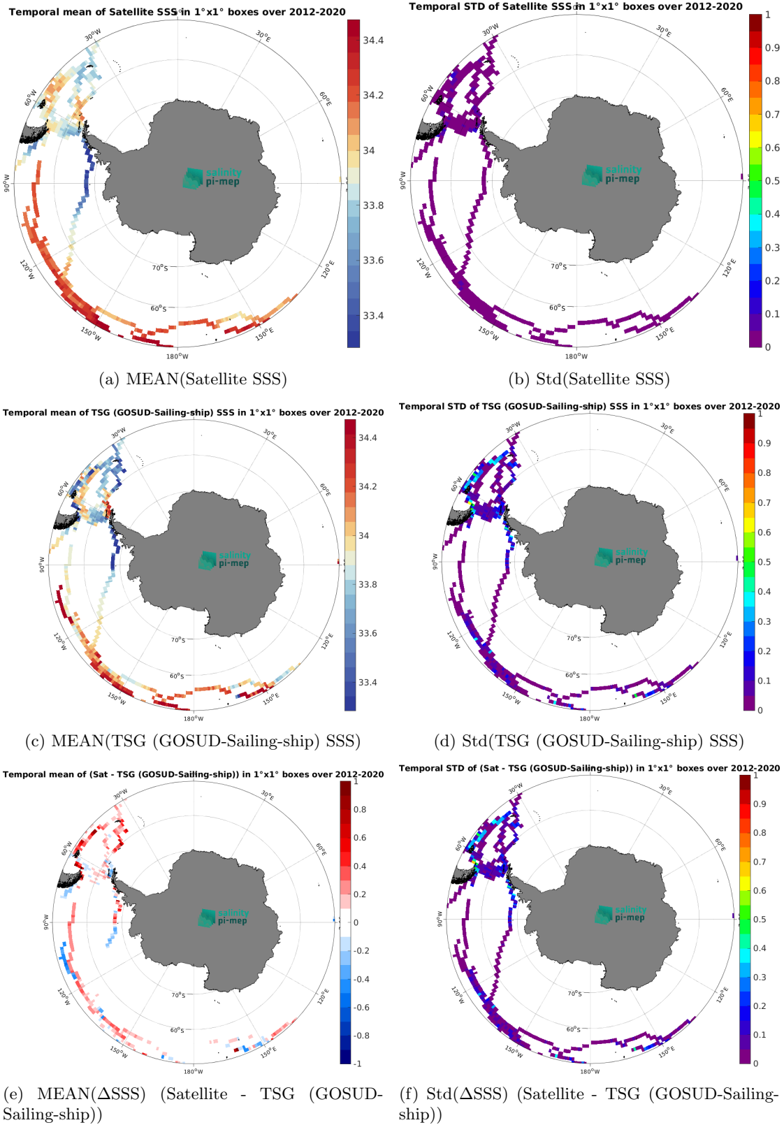
Figure 7: Temporal mean (left) and Std (right) of SSS from SMAP SSS L4 OI v3 - Monthly (ESR) (top), TSG (GOSUD-Sailing-ship) (middle), and of \Delta SSS (Satellite - TSG (GOSUD-Sailing-ship)). Only match-up pairs are used to generate these maps.
