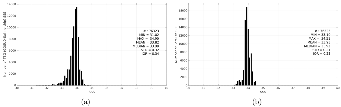
Figure 3: Histograms of SSS from TSG (GOSUD-Sailing-ship) (a) and SMAP SSS L4 OI v3 - Monthly (ESR) (b) considering all match-up pairs per bins of 0.1 over the Southern Ocean Pi-MEP region and for the full satellite product period.
