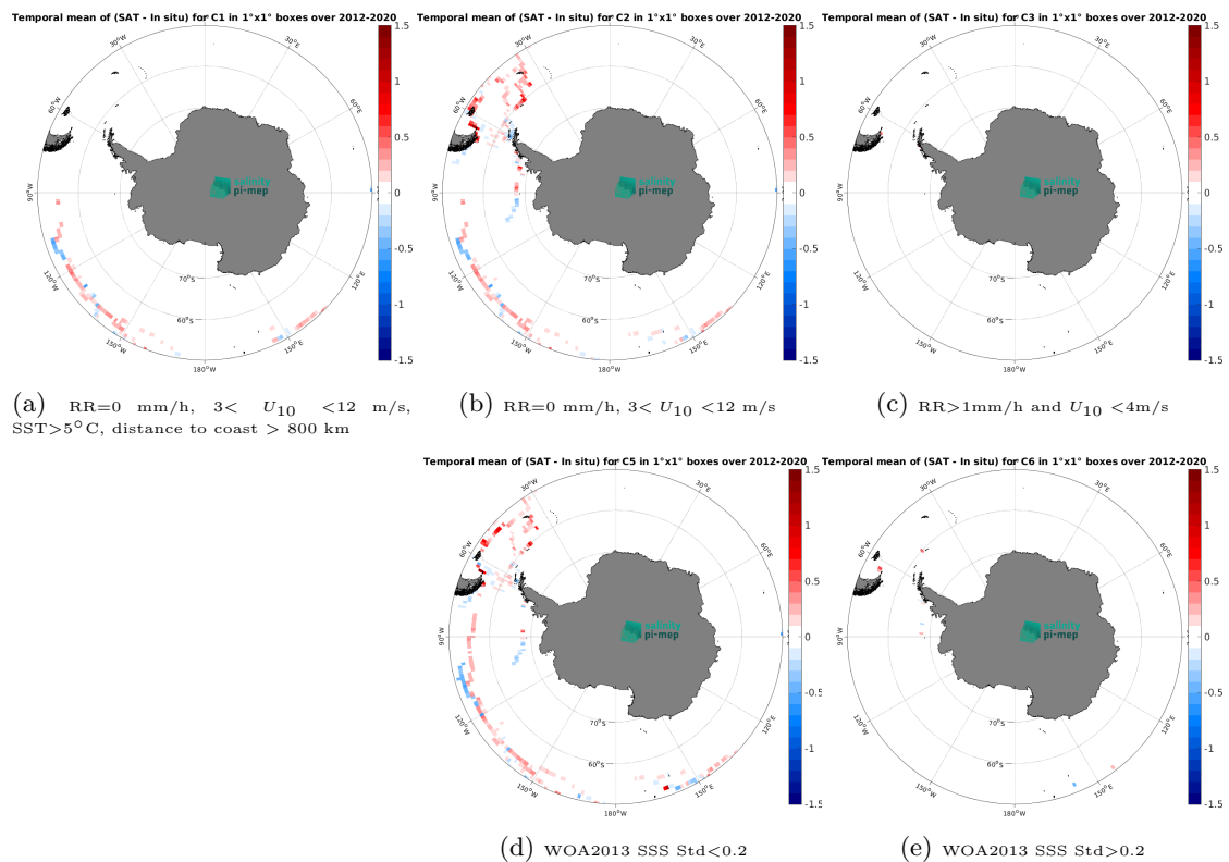
Figure 14: Temporal mean gridded over spatial boxes of size 1^\circ \times 1^\circ of \Delta SSS (SMAP SSS L4 OI v3 - Monthly (ESR) - TSG (GOSUD-Sailing-ship)) for 5 different subdatasets corresponding to: RR=0 mm/h, 3 < U_{10} < 12 m/s, SST >5^\circ C, distance to coast > 800 km (a), RR=0 mm/h, 3 < U_{10} < 12 m/s (b), RR >1 mm/h and U_{10} < 4 m/s (c), WOA2013 SSS Std <0.2 (d), WOA2013 SSS Std >0.2 (e).
