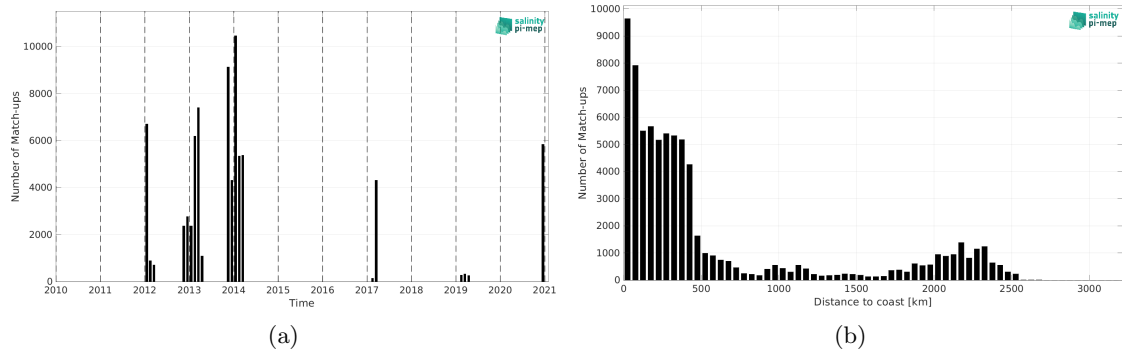
Figure 2: Number of match-ups between TSG (GOSUD-Sailing-ship) and SMAP SSS L4 OI v3 - Monthly (ESR) SSS as a function of time (a) and as function of the distance to coast (b) over the Southern Ocean Pi-MEP region and for the full satellite product period.
