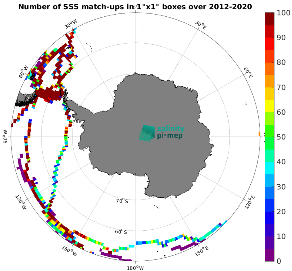
Figure 5: Number of SSS match-ups between TSG (GOSUD-Sailing-ship) SSS and the SMAP SSS L4 OI v3 - Monthly (ESR) SSS product for the Southern Ocean Pi-MEP region over 1^{\circ} \times 1^{\circ} boxes and for the full satellite product period.
