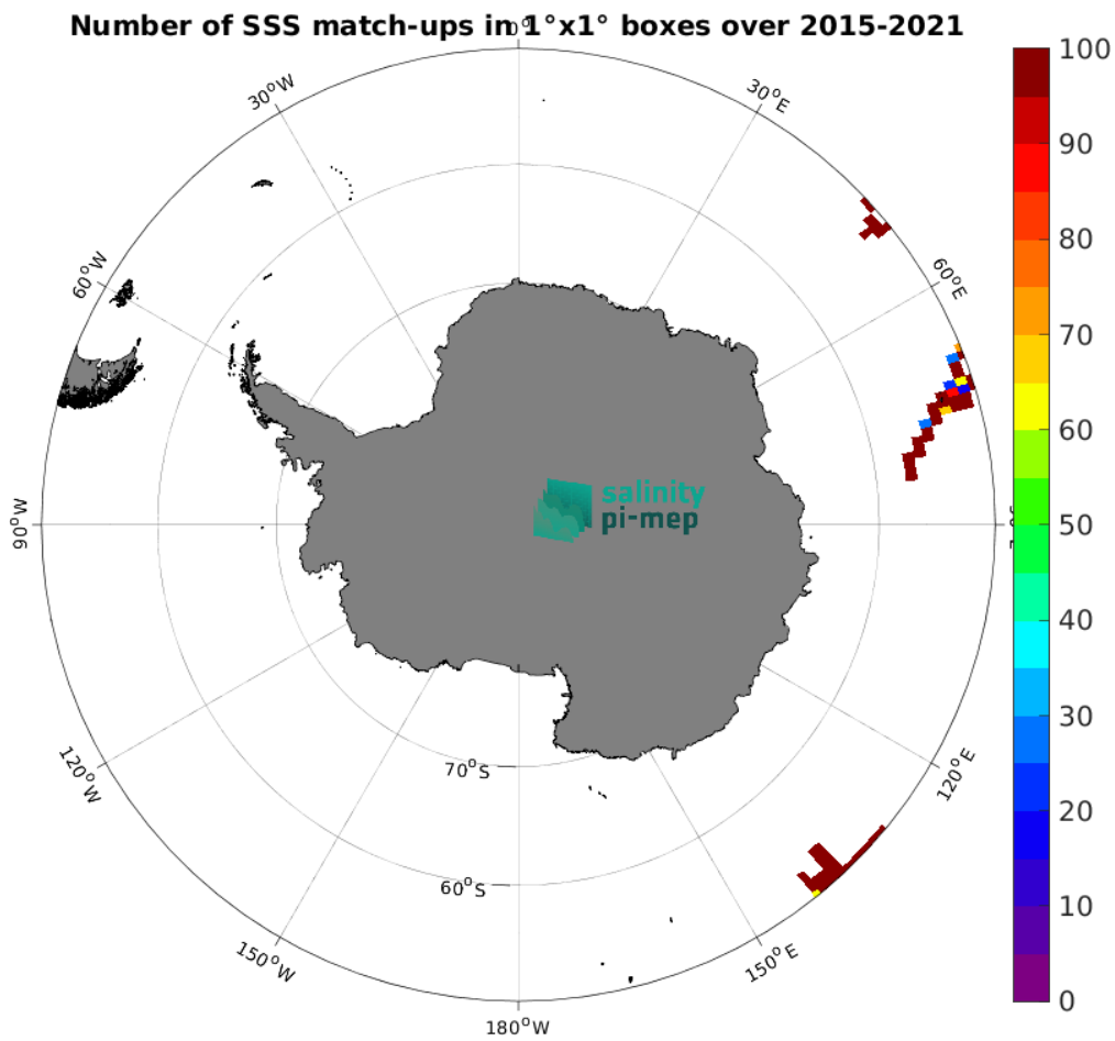
Figure 5: Number of SSS match-ups between TSG (GOSUD-Research-vessel) SSS and the SMAP SSS L4 OI v3 - Monthly (ESR) SSS product for the Southern Ocean Pi-MEP region over 1^\circ \times 1^\circ boxes and for the full satellite product period.
