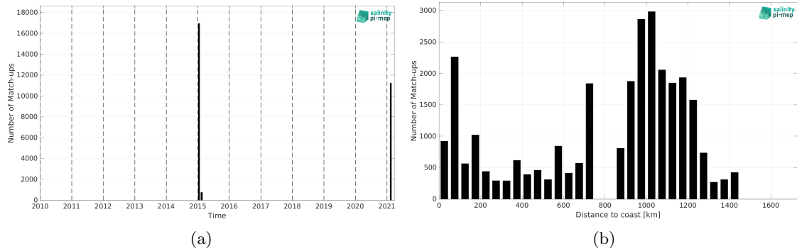
Figure 2: Number of match-ups between TSG (GOSUD-Research-vessel) and SMAP SSS L4 OI v3 - Monthly (ESR) SSS as a function of time (a) and as function of the distance to coast (b) over the Southern Ocean Pi-MEP region and for the full satellite product period.
