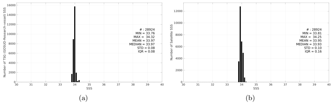
Figure 3: Histograms of SSS from TSG (GOSUD-Research-vessel) (a) and SMAP SSS L4 OI v3 - Monthly (ESR) (b) considering all match-up pairs per bins of 0.1 over the Southern Ocean Pi-MEP region and for the full satellite product period.
