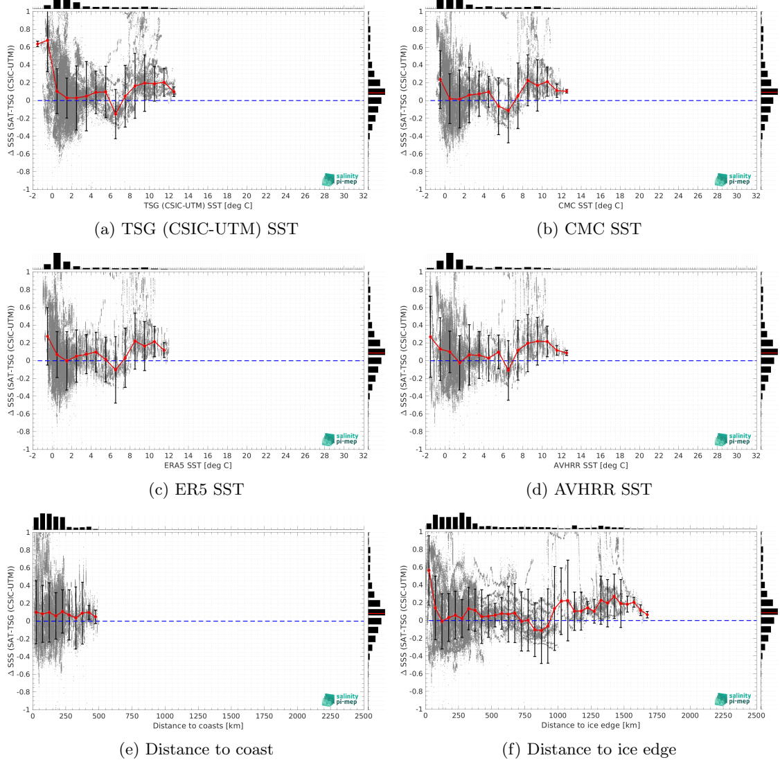
Figure 13: \Delta SSS (Satellite - TSG (CSIC-UTM)) sorted as function of TSG (CSIC-UTM) SST values (a), CMC SST (b), ERA5 SST (c), AVHRR SST (d), distance to coast (e) and distance to ice edge (f). In all plots the median and Std of \Delta SSS for each bin is indicated by the red curves and black vertical thick bars ( \pm 1 Std). Links to similar figures sorted as function of Sea ice fraction and in situ measurement depth .
