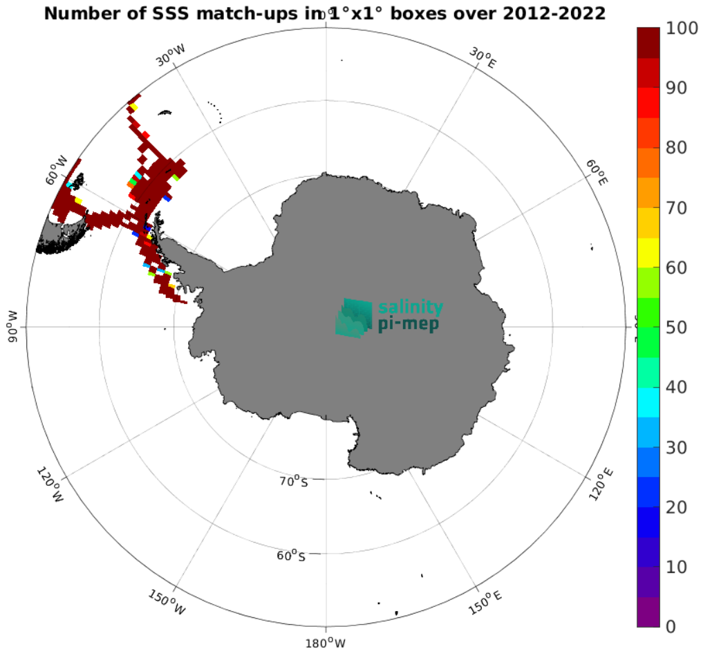
Figure 5: Number of SSS match-ups between TSG (CSIC-UTM) SSS and the SMAP SSS L4 OI v3 - Monthly (ESR) SSS product for the Southern Ocean Pi-MEP region over 1^\circ \times 1^\circ boxes and for the full satellite product period.
